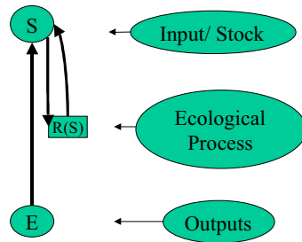
Figure 3: Ecological system
