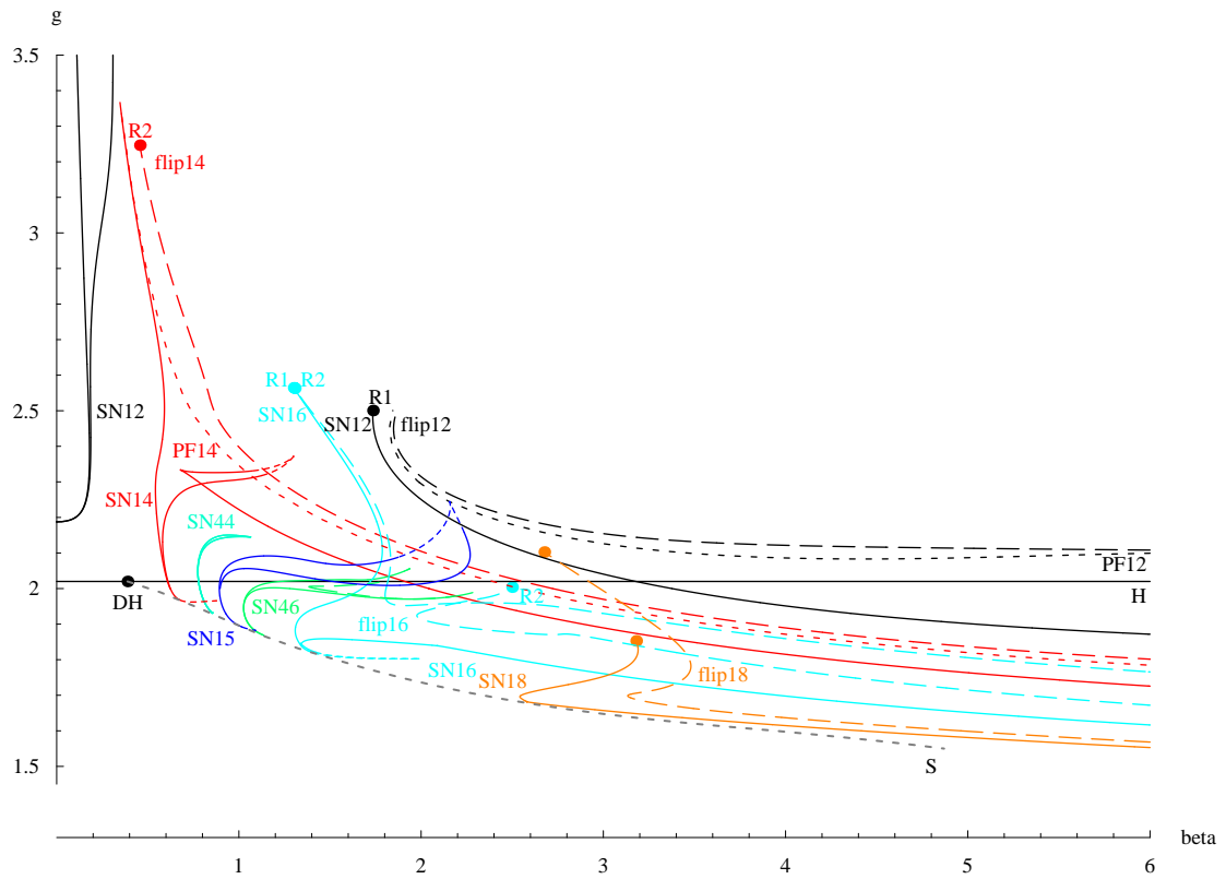
Figure 7: Bifurcation diagram in the \beta - g -plane for v = 0.6 . The point DH is a Chenciner bifurcation point, lying on the Hopf bifurcation line H: g = 2R . The lower dashed line S starting at the Chenciner bifurcation point corresponds to the saddle-node bifurcation curve of invariant circles. PF n denotes pitchfork bifurcations curves of points of period n , which are indicated by short dashes; further notation as in figure 6.
