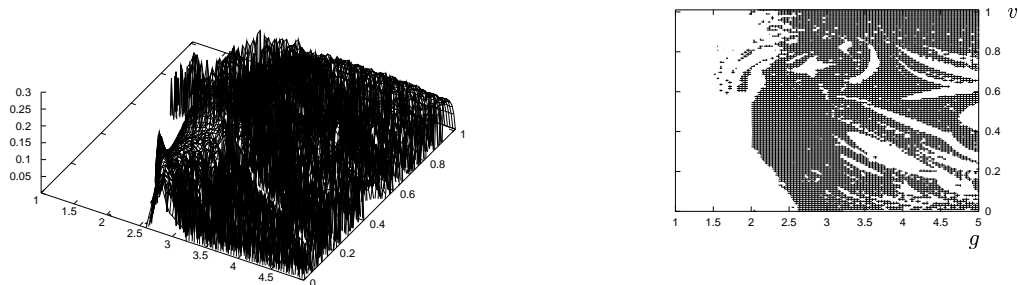
Figure 9: Lyapunov exponents for g \in [1, 5] , v \in [0, 1] , \beta = 3 : on the left, the magnitude of the upper Lyapunov exponent is plotted along the z -axis. In the right picture, for points in the grey area, upper Lyapunov exponents are positive – for those parameters, there is a chaotic attractor (compare the bifurcation diagram in figure 6).
