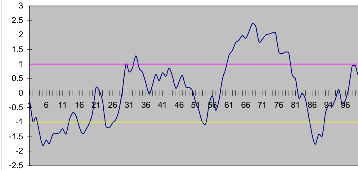
Figure 1: Simulated Exchange Rate Data from the DAWOP Model
