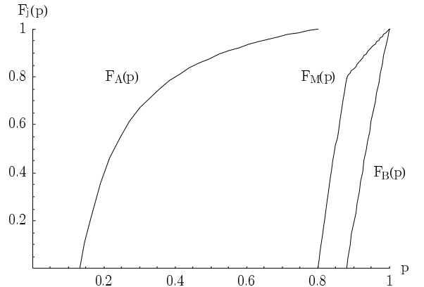
Figure 5b. High \beta ( \gamma = 1/20; \beta = 8 ).
