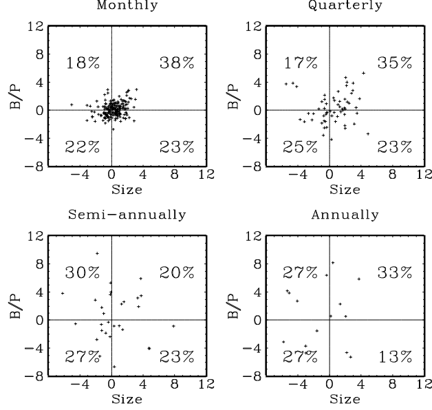
Figure 2: Scatter diagrams of cross-sectionally estimated coefficients The figures contains scatter diagrams of the estimated coefficients per cross-section of a regression of future excess returns in excess of an equally weighted portfolio on Size and Book-to-Price (B/P). The percentages give the fraction of coefficient couples (Size,B/P) present in the quadrant.
