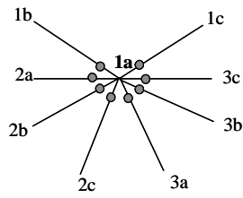
Figure 3: Center-Sponsored Star
