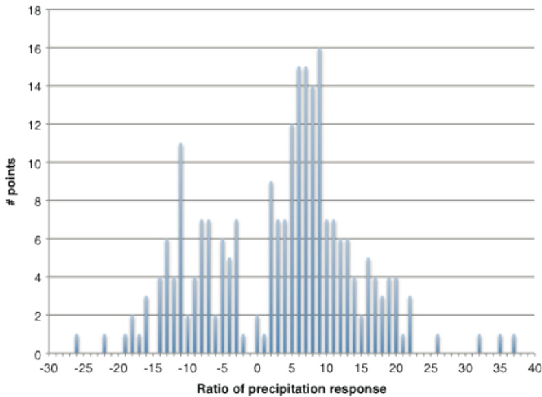
Figure 4. The ratio of precipitation changes in response to forcing by BC and co-emitted species relative to equal global mean LLGHG forcing. Values are from analysis of ~250 land locations from 60°S–60°N where responses were statistically significant in both sets of simulations [Shindell et al. , 2012a].
