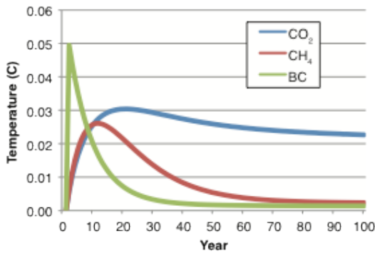
Figure 3. Timescales of temperature response to different forcers (°C per kg x 1 year’s worth of current global anthropogenic emissions (excluding open biomass burning)).
