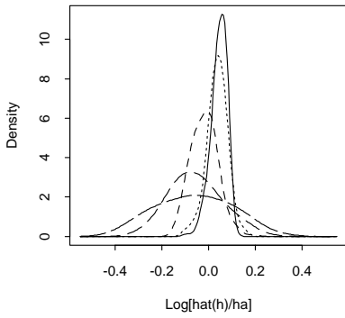
Figure 2i: m=1, \phi_1=0.3 , all delta's
