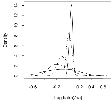
Figure 2j: \phi_1=0.7 , all delta's
