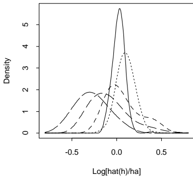
Figure 2: Kernel densities of \log(\hat{h}/h_A) for AlgB with g_2 & n = 500 ( g_2 is shown in Fig. 2k).
