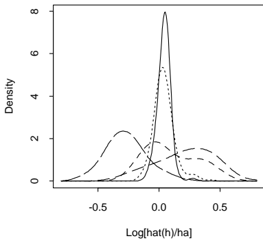
Figure 2f: m=1, \phi_1=-0.7 , all delta's
