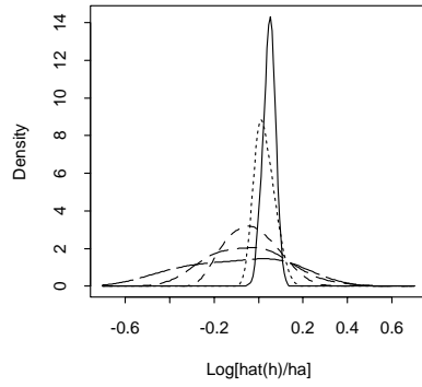
Figure 2e: m=0, \phi_1=0.7 , all delta's
