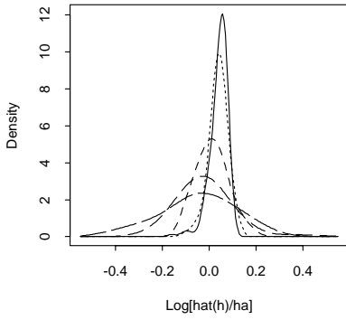
Figure 2d: m=0, \phi_1=0.3 , all delta's
