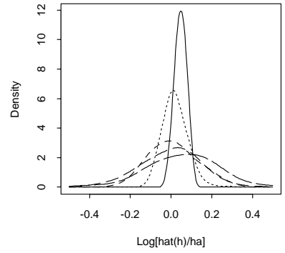
Figure 2c: m=0, \phi_1=0.0 , all delta's
