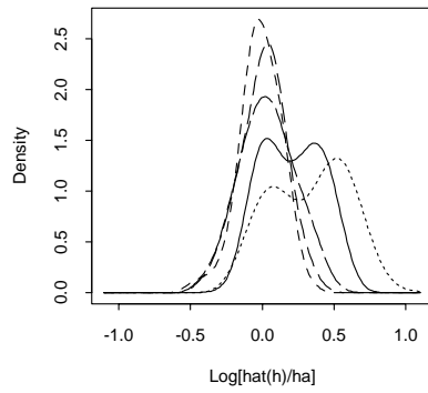
Figure 2g: m=1, \phi_1=-0.3 , all delta's
