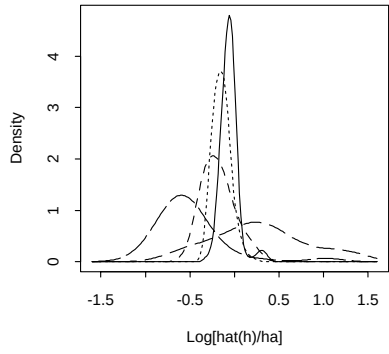
Figure 4f: m=1 , \phi_1=-0.7 , all \delta 's
