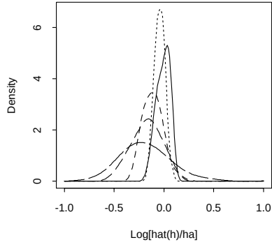
Figure 4d: m=0 , \phi_1=0.3 , all \delta 's
