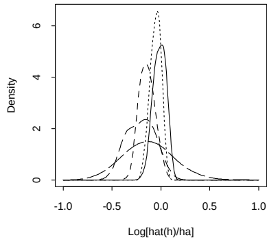
Figure 4i: m=1 , \phi_1=0.3 , all \delta 's
