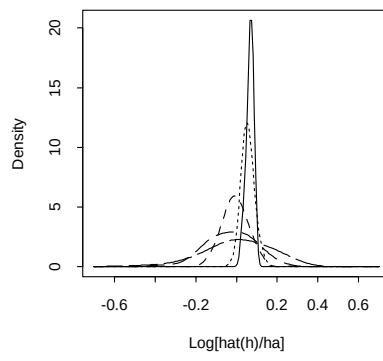
Figure 11e: m=0 , \phi_1=0.7 , all delta's
