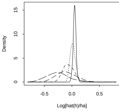
Figure 11: Kernel densities of \log(\hat{h}/h_A) for AlgC with g_2 and n = 1000 .
