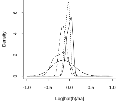
Figure 10i: m=1 , \phi_1=0.3 , all delta's
