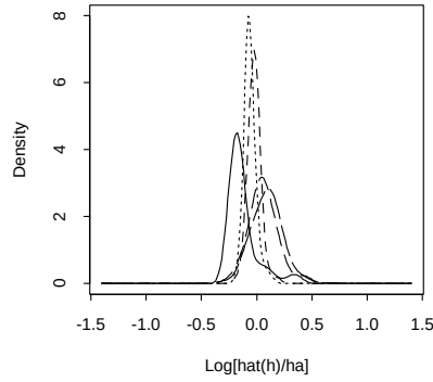
Figure 12: Kernel densities of \log(\hat{h}/h_A) for AlgC with g_3 and n = 1000 .
