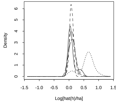
Figure 6g: m=1 , \phi_1=-0.3 , all \delta 's
