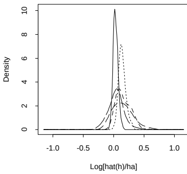
Figure 9: Kernel densities of \log(\hat{h}/h_A) for AlgC with g_3 and n = 500 .
