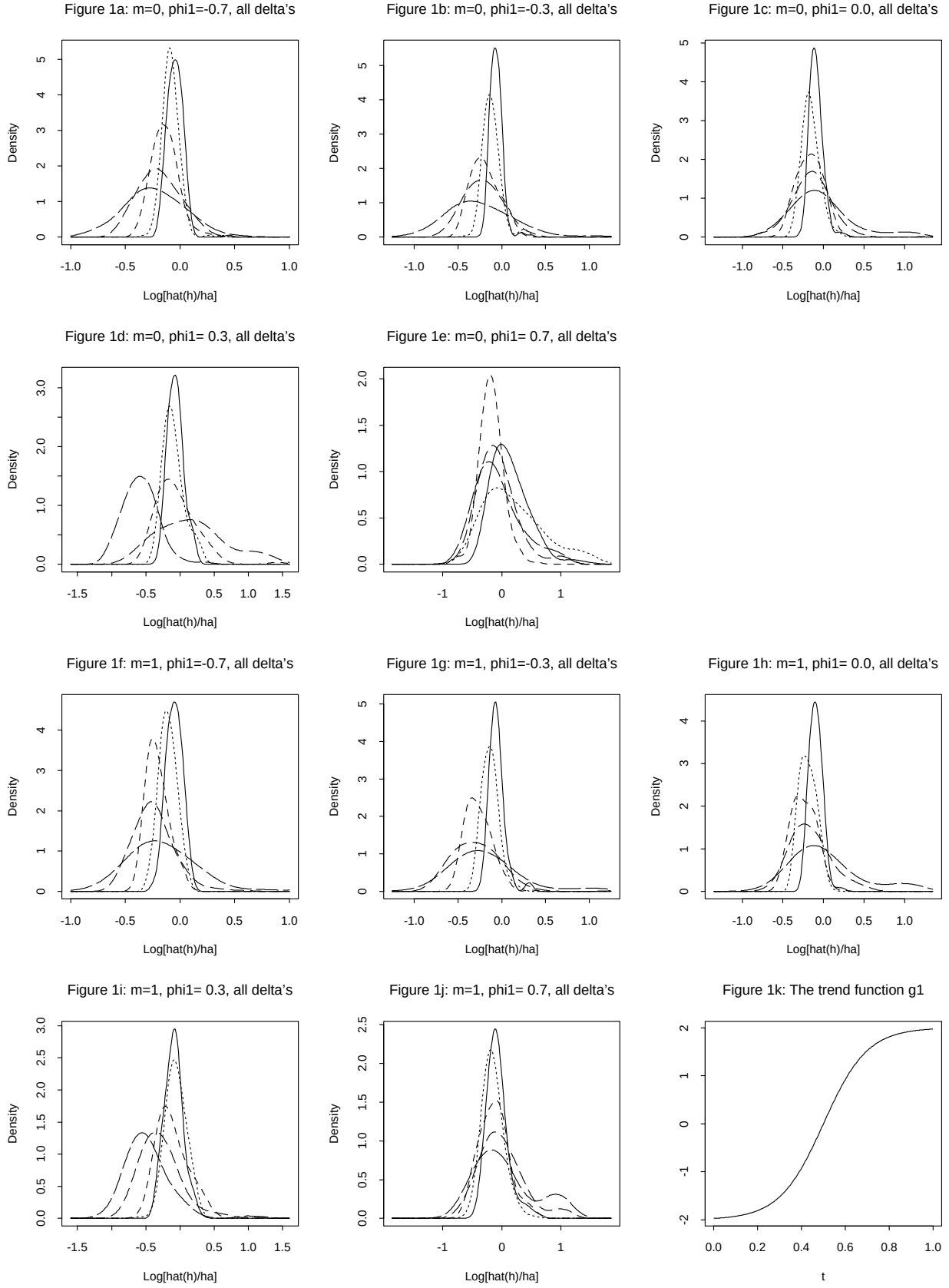
Figure 1: Kernel densities of \log(\hat{h}/h_A) for AlgB with g_1 & n = 500 ( g_1 is shown in Fig. 1k).
