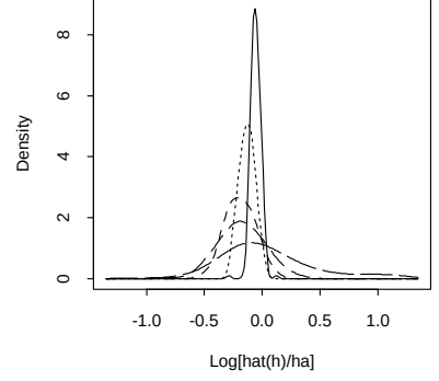
Figure 10h: m=1 , \phi_1=0.0 , all delta's
