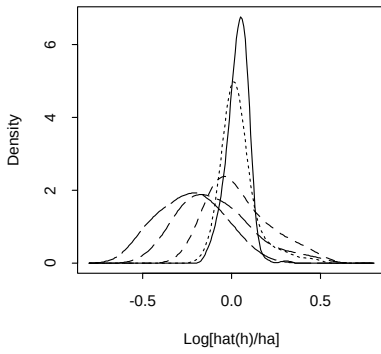
Figure 8: Kernel densities of \log(\hat{h}/h_A) for AlgC with g_2 and n = 500 .
