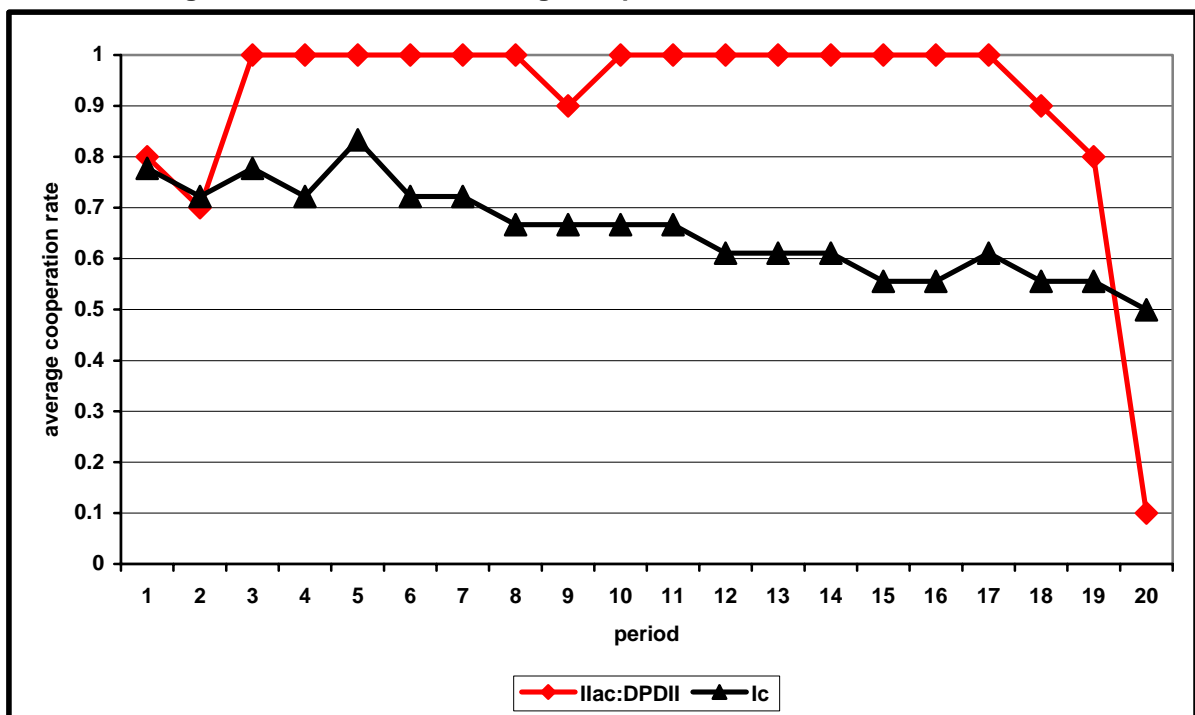
Figure 4: Time series of average cooperation rates in Ic and Ilac:DPDII
