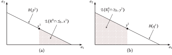
Figure 3: An illustration of \tilde{R}_J and \tilde{R} . In (a), we have x^1 R^0 a and x^1 \succ_S a for all a in the indicated region and thus x^1 \tilde{R}_J a . In (b), we have y^1 R_J^0 a and y^1 \succ_S a for all a in the indicated region and thus y^1 \tilde{R} a .
