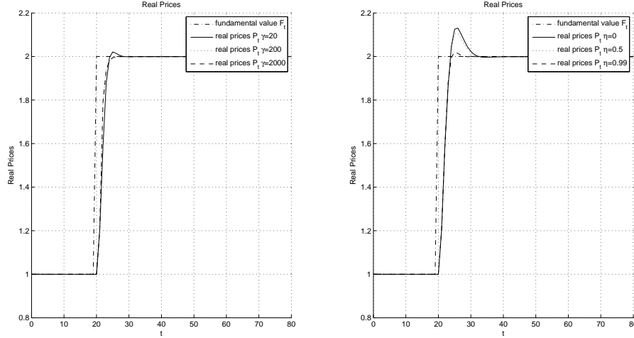
Figure 6: Price reaction to a step shock in news fundamentals in the complex model with L_l = 4 , \mu = 1.4 , and variation of rationality \gamma and memory \eta
