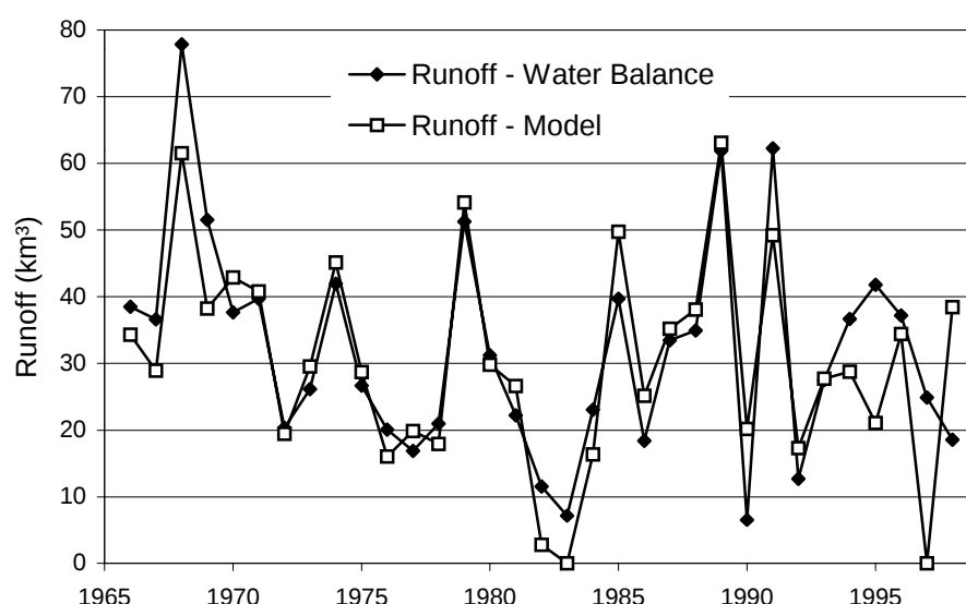
Figure 7: Runoff into Akosombo Reservoir
