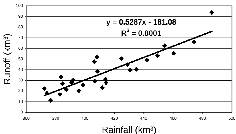
Figure 2: Runoff as a Function of Rainfall (1936-1963)
