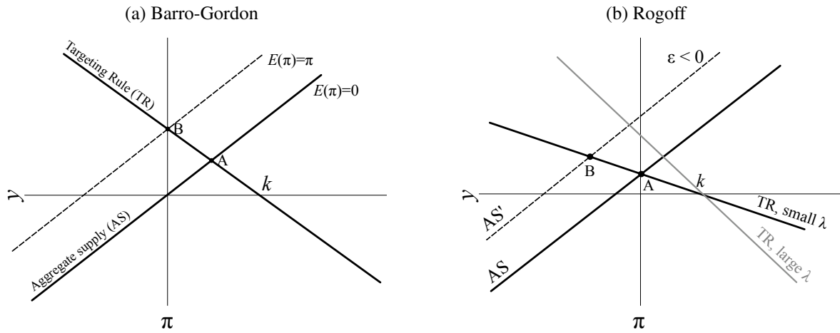
Figure 1: Graphical representation of the Barro-Gordon and Rogoff models
