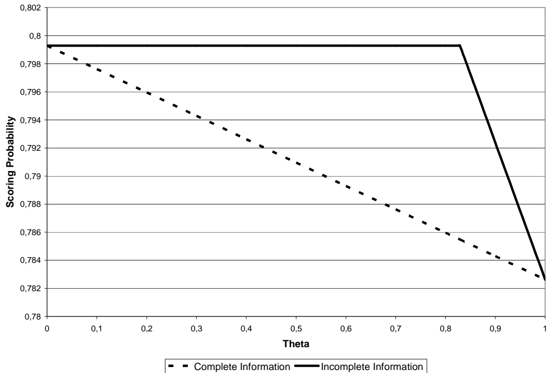
Figure 4: Average scoring probabilities (three-strategy model)
