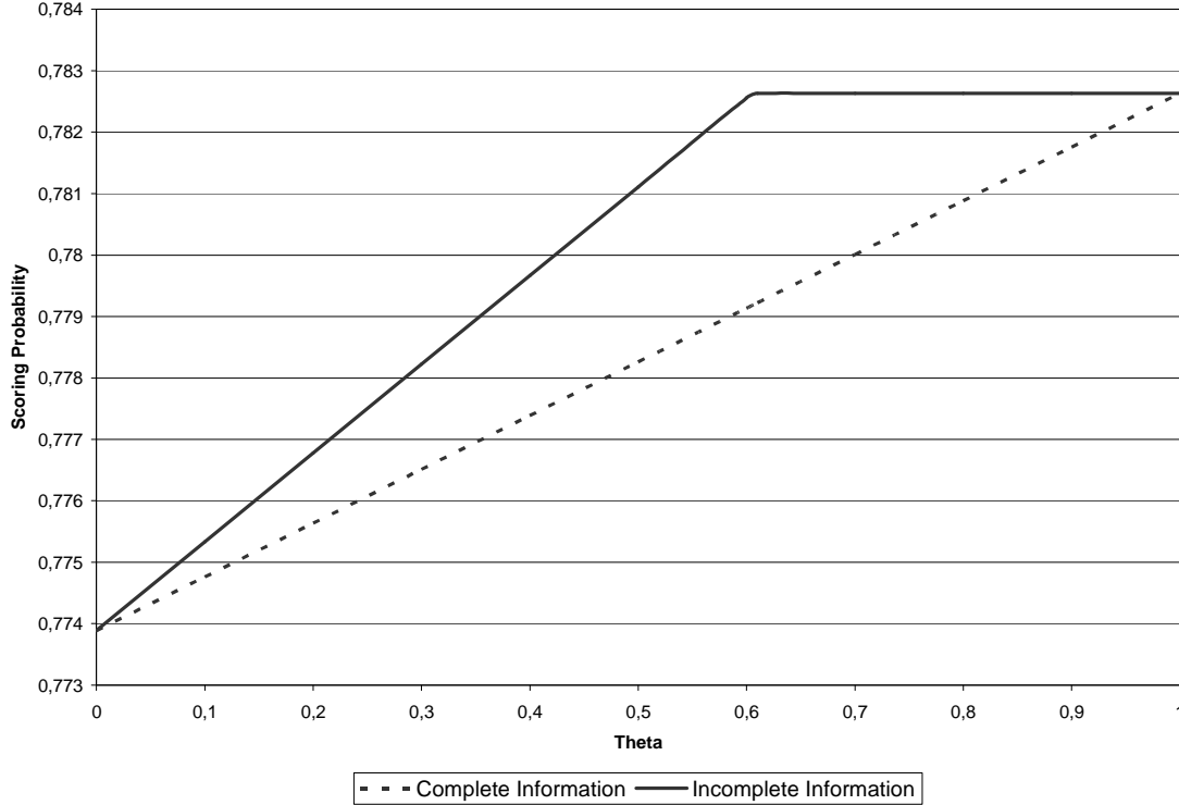
Figure 2: Average scoring probabilities (two-strategy model)
