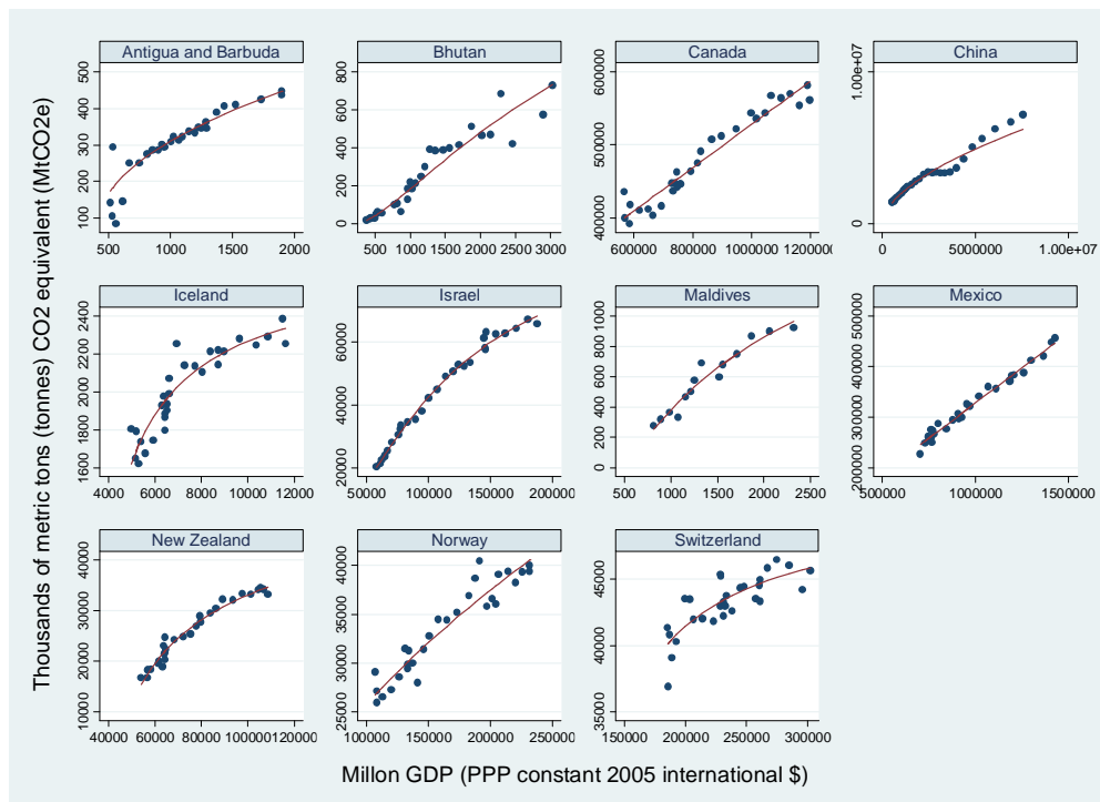
Figure 1. Relationship between emissions and GDP by country: functional forms
