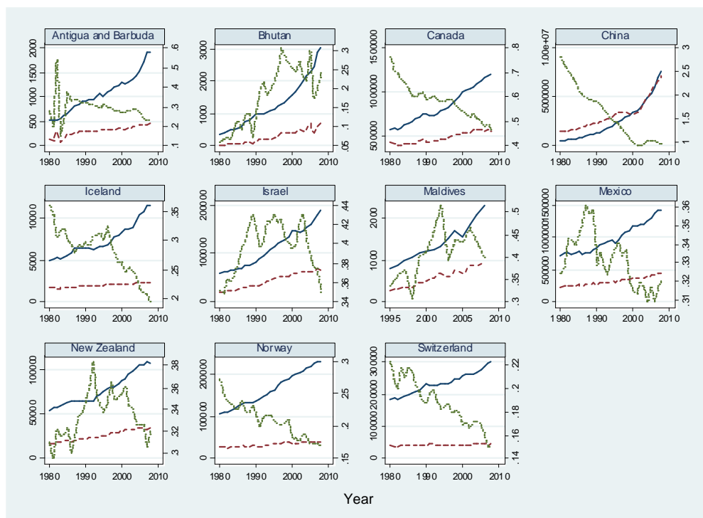
Figure 1.A. GDP, CO 2 emissions and emissions intensity by country
