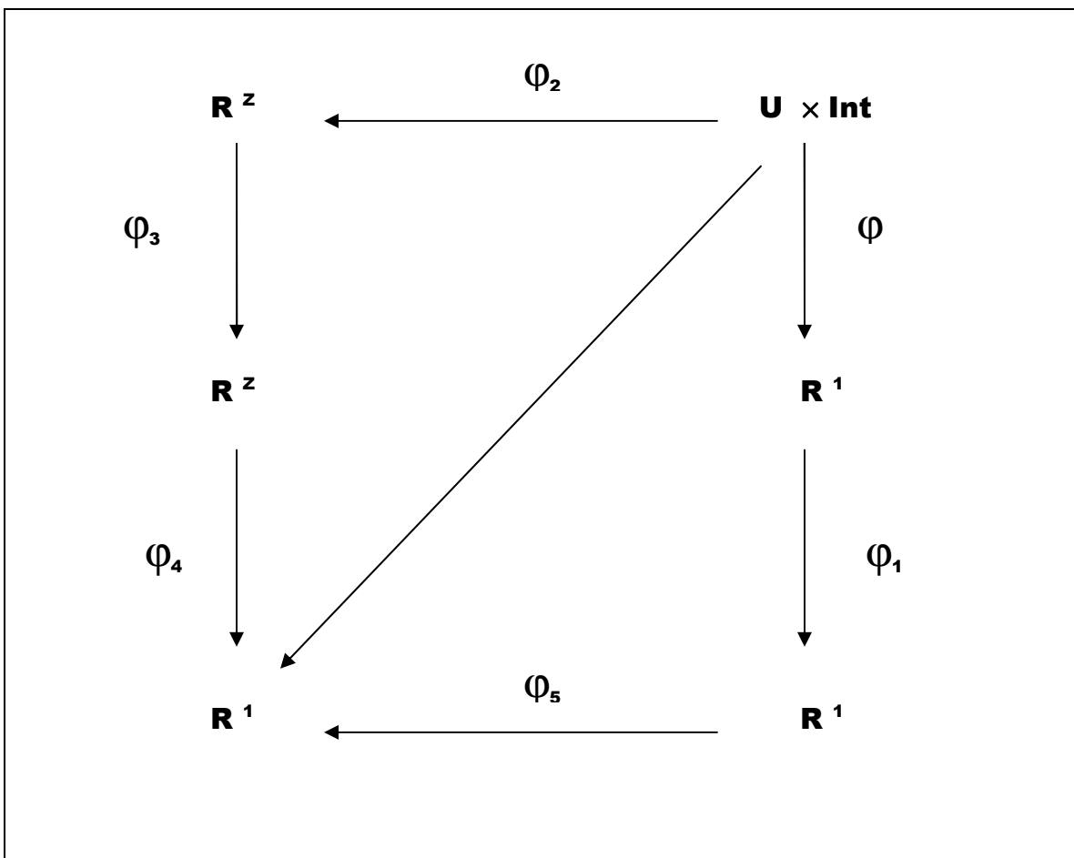
Exhibit 1 The commutative diagram brought about by the multiplicative model
