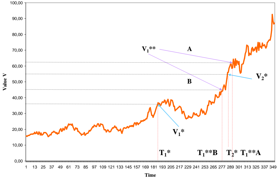
Graph 1 Simulated dynamics for state variable V and trigger values for decisions
