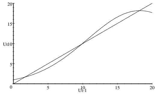
UK Phase Diagram
