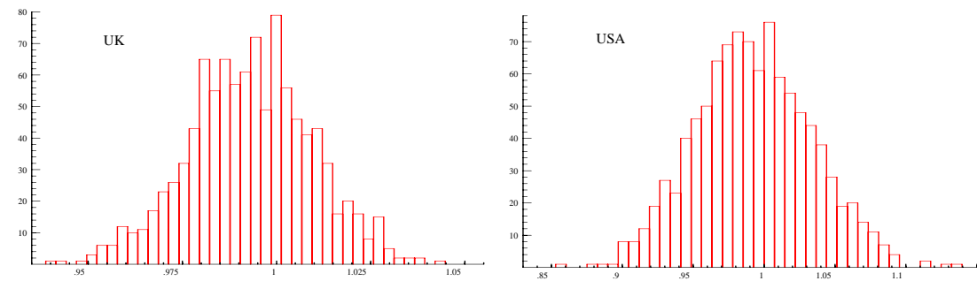
Fig. 5. Countries Distribution over \sigma
