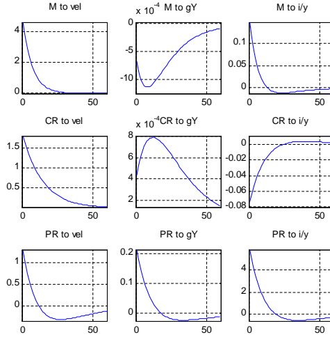
Figure 1: Impulse Responses: Velocity, Output Growth, Investment Ratio
