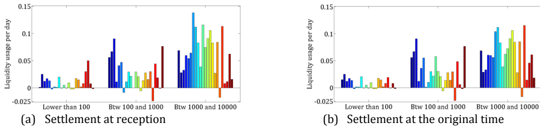
Figure 5. Average additional liquidity usage per day
