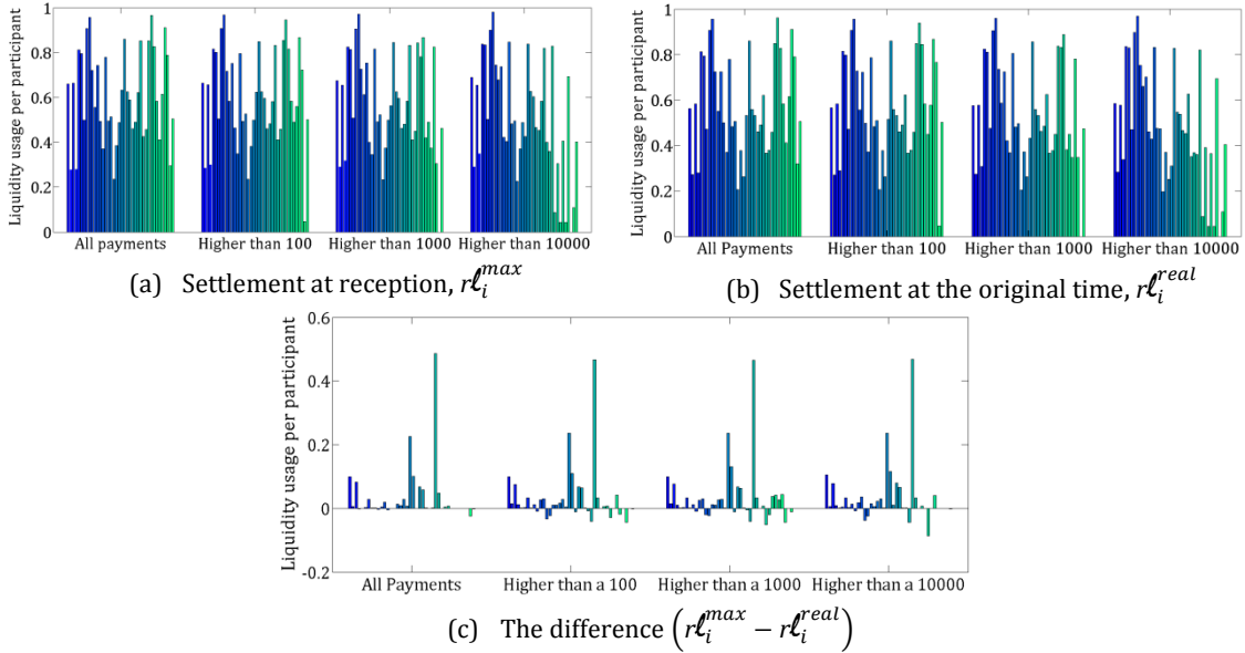
Figure 1. The average proportional liquidity usage per participant
