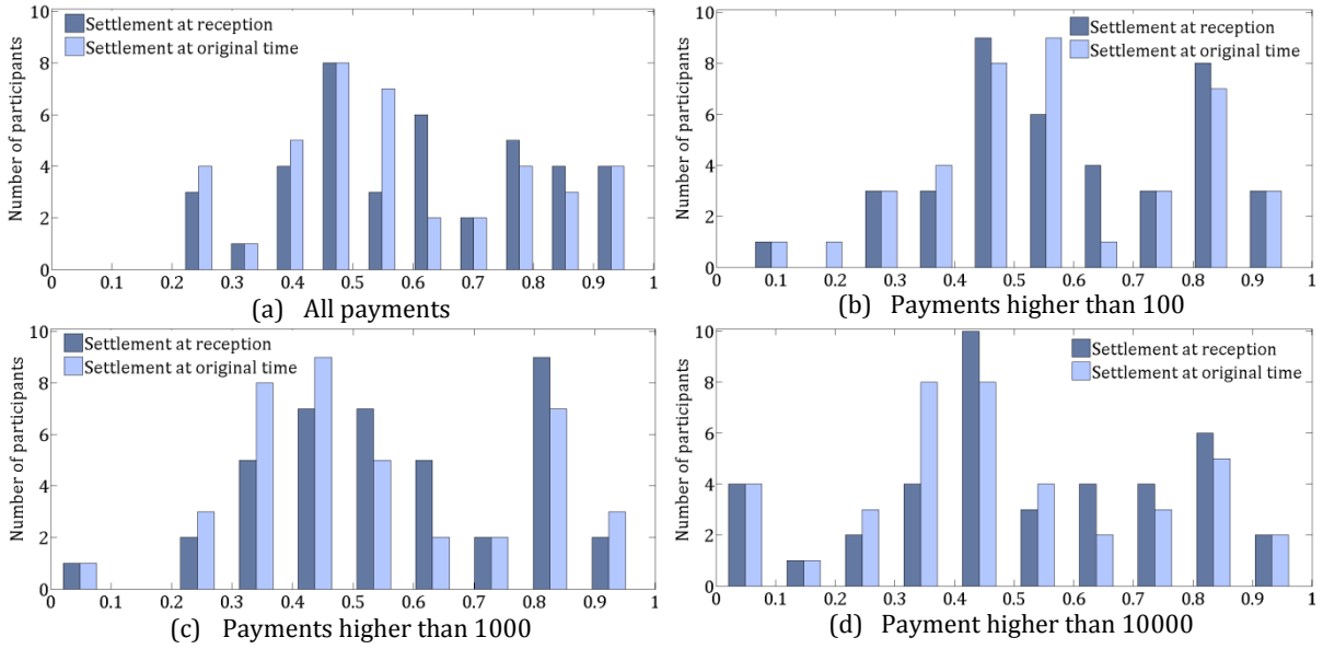
Figure 2. The histogram of the average proportional liquidity usage per participant
