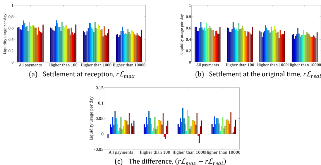
Figure 4. Proportional average liquidity usage per day
