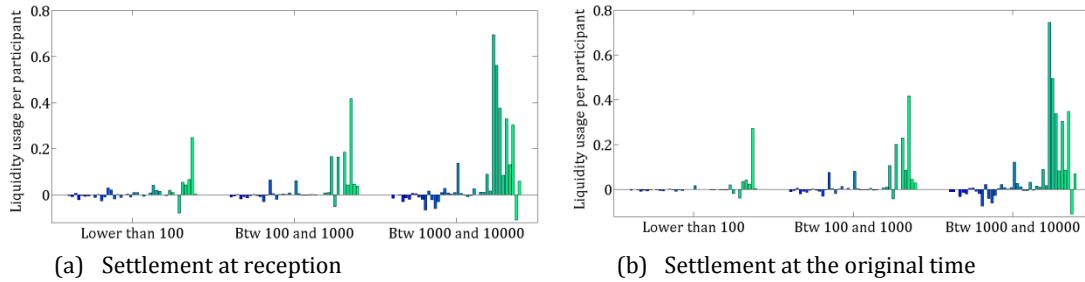
Figure 3. Average additional liquidity usage per participant
