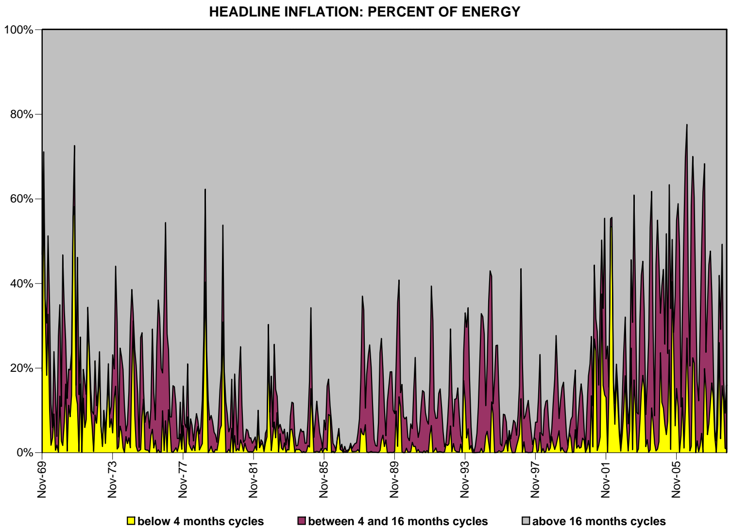
Figure 14. Energy decomposition for headline inflation through time. The energy of each scale is expressed as fraction of the overall energy.
