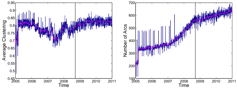
(a) Daily average clustering coefficient
