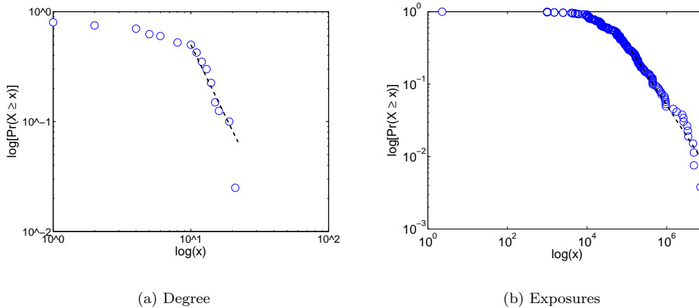
Figure 10: Test for the power law distribution for the base case network (without CLS)
