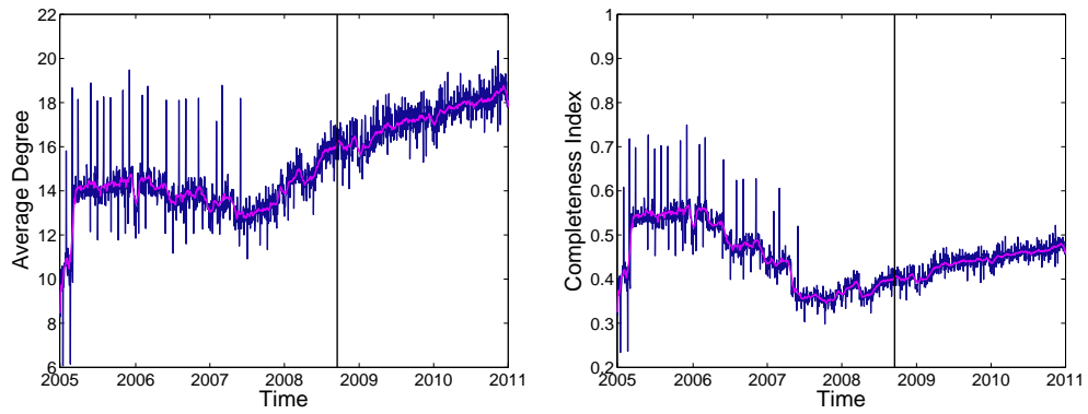
(a) Daily Average degree
