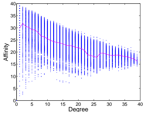
(a) Affinity vs degree
