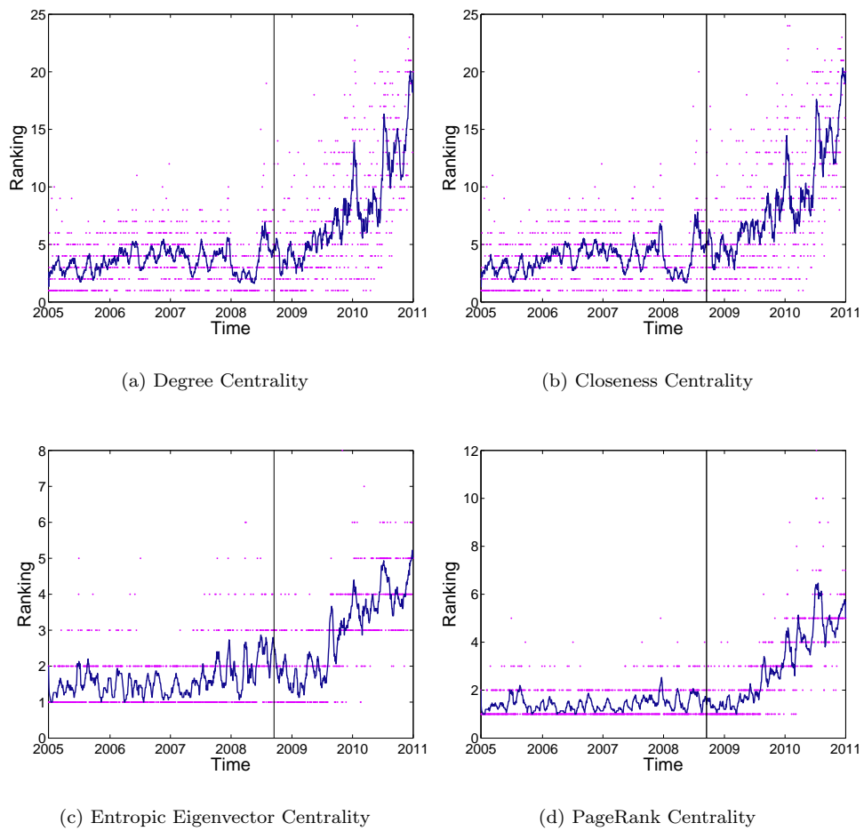
Figure 17: Individual centrality measures.
