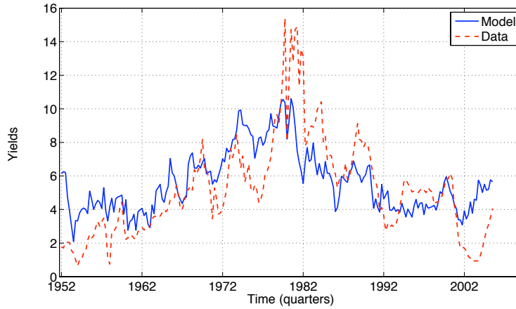
Figure 12: The short term rate for specification H.
