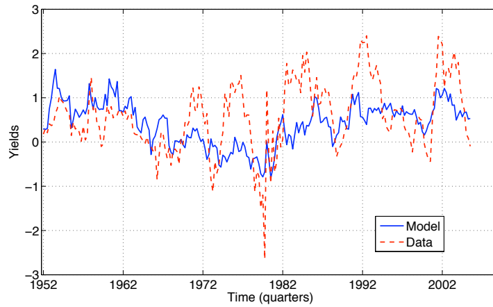
Figure 13: The yields spread for specification H.
