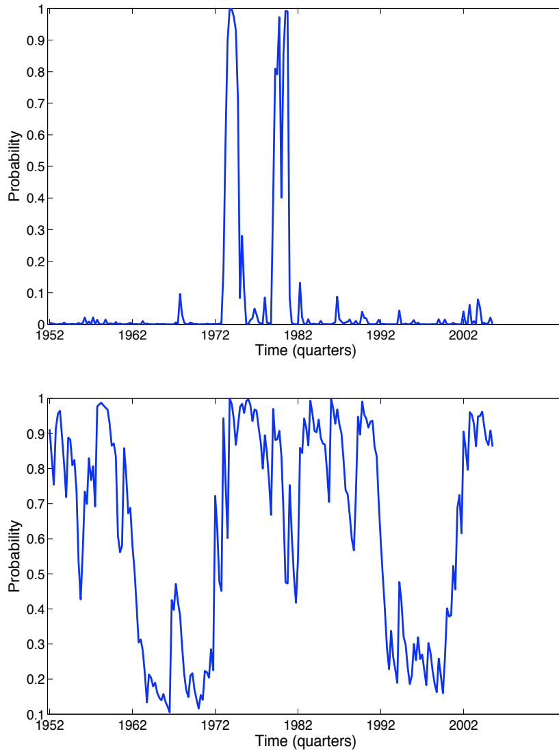
Figure 20: Estimates of the probability regime states for specification \Gamma_2 .
