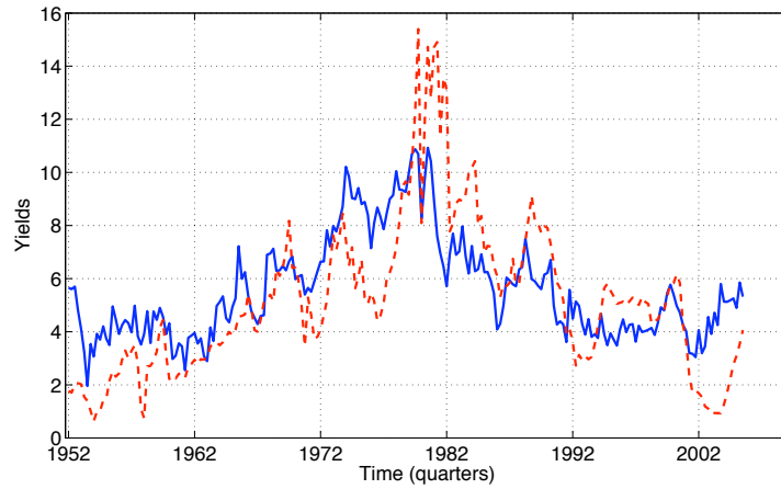
Figure 15: The short term rate for specification \mathbf{I}' .
