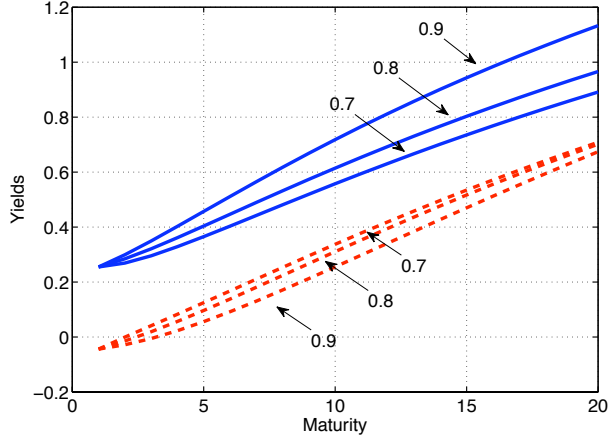
Figure 11: Function F(n, s_{2,t})/n for different levels of persistence.
