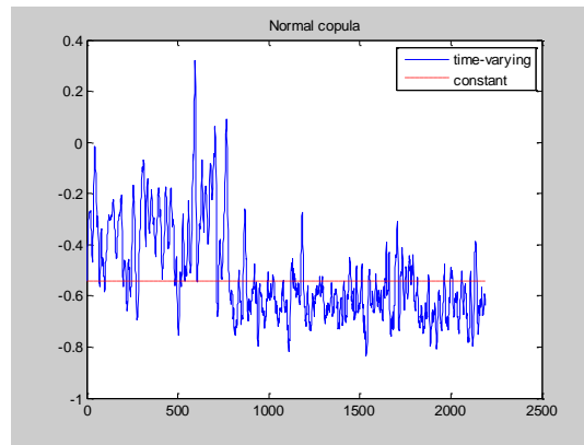
Figure 5 – Time-varying copula
