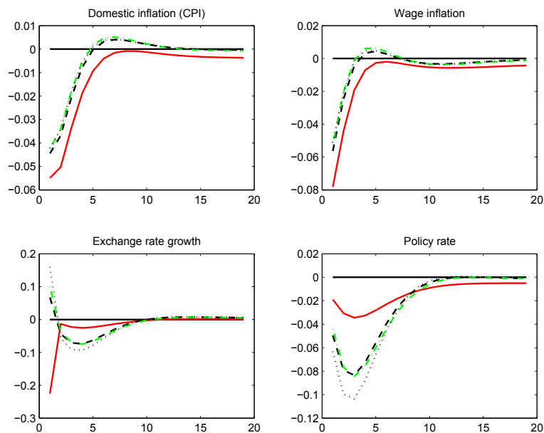
Figure 9 Productivity shock (EMP solid, OSR1 dashed, OSR2 dotted, OSR3 dashed-dotted)
