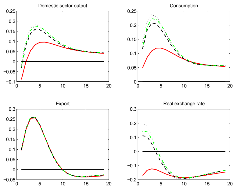
Figure 10 Productivity shock (EMP solid, OSR1 dashed, OSR2 dotted, OSR3 dashed-dotted)
