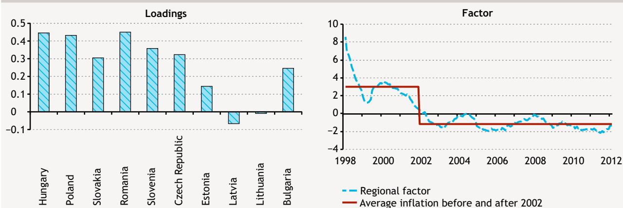
Chart 8 The first regional factor and its loadings
