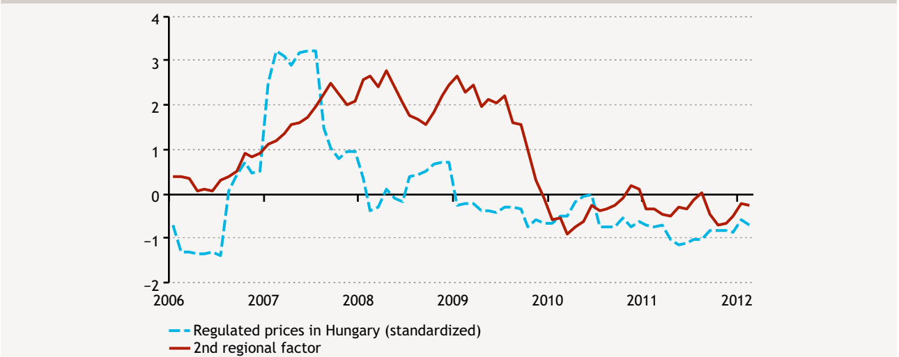
Chart 10 Regulated prices in Hungary and the second regional factor
