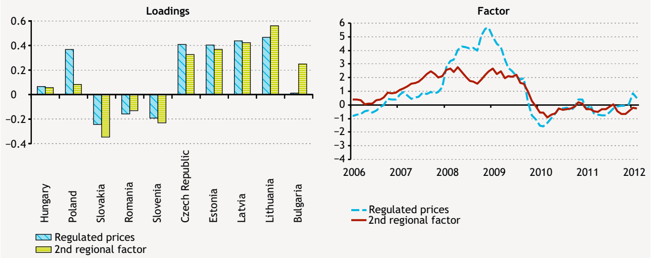
Chart 9 Principal components of regulated prices and the second regional factor
