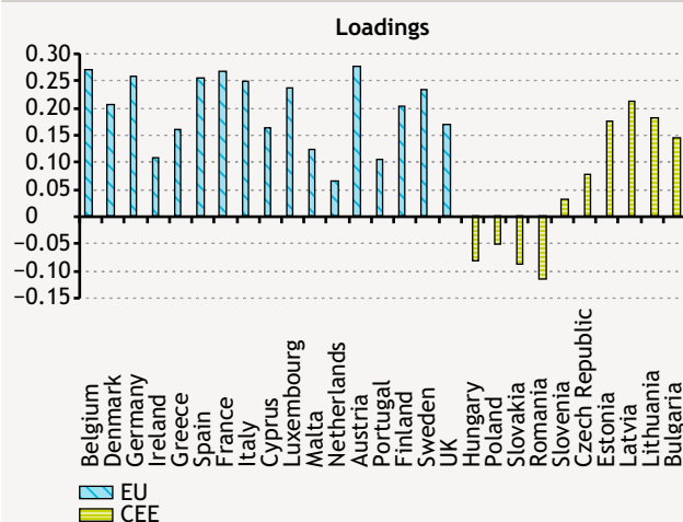
Chart 17 Common factor before the crisis
