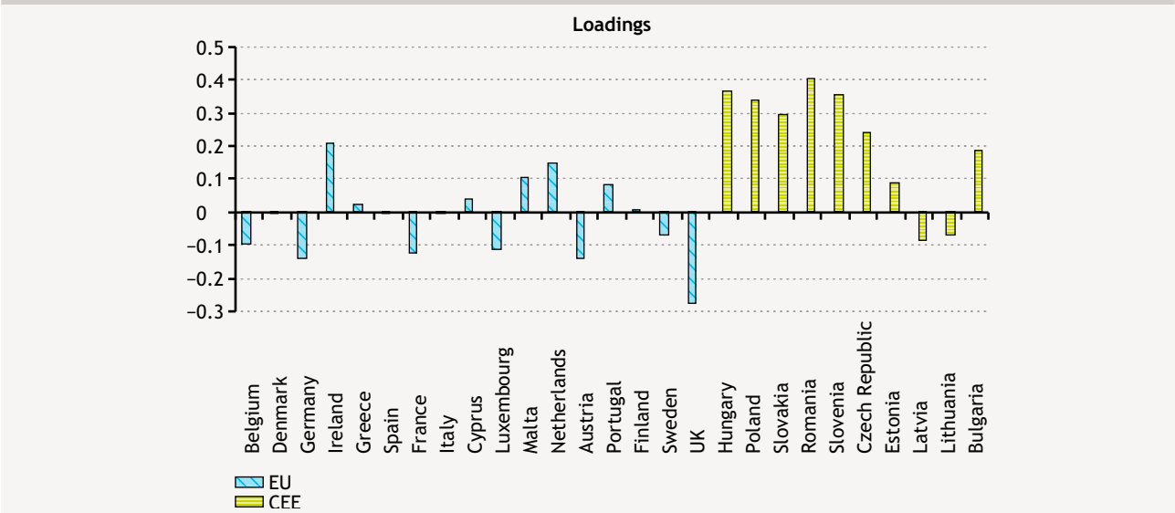
Chart 6 Loadings of the second common factor
