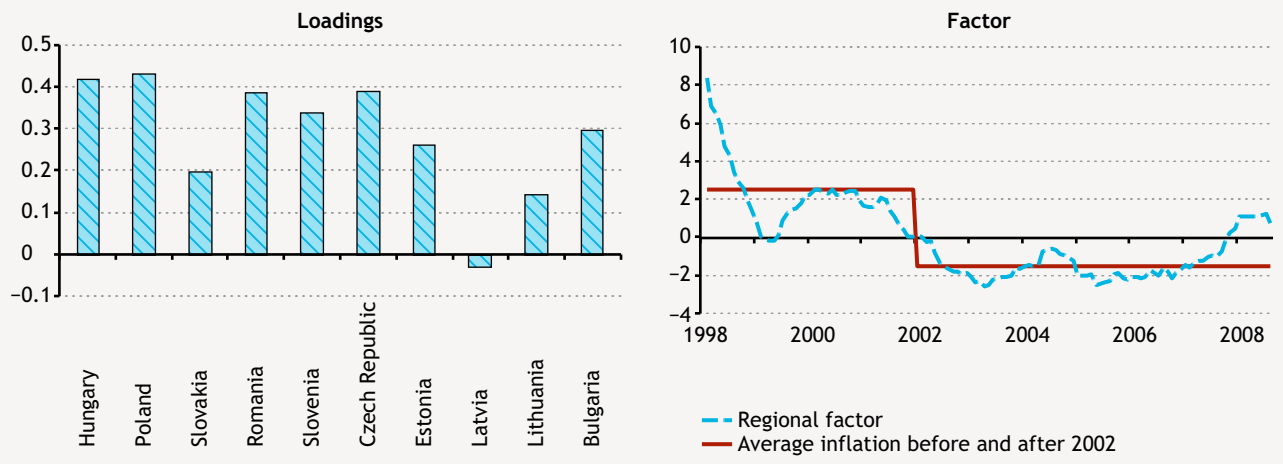
Chart 18 Regional factor before the crisis
