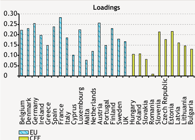
Chart 15 Common factor with monthly changes
