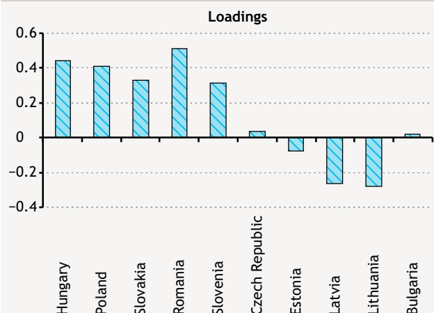
Chart 16 Regional factor with monthly changes
