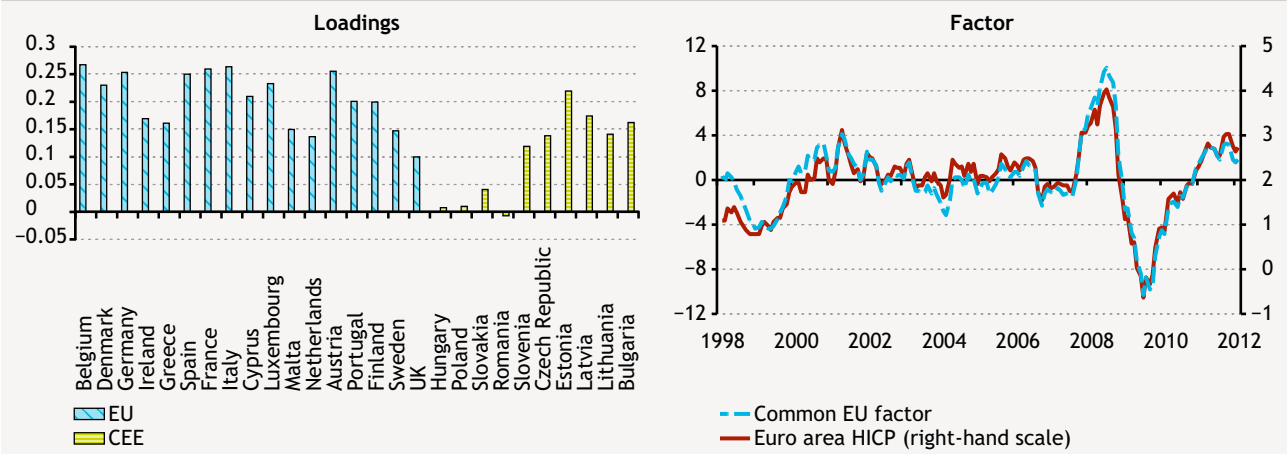
Chart 5 The first common factor and its loadings
