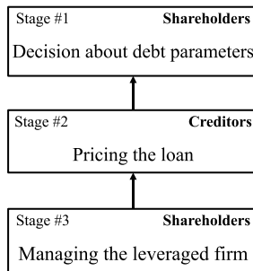
Figure 5: The game tree of the loan agreement
