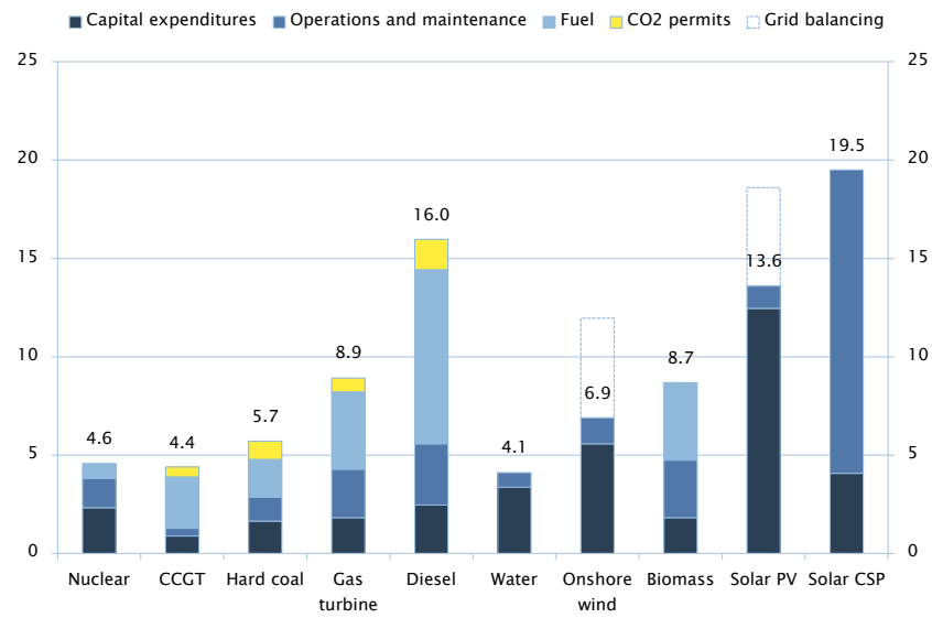
Figure 2: Estimated unit electricity costs in EUR/MWh according to BCG [12].
