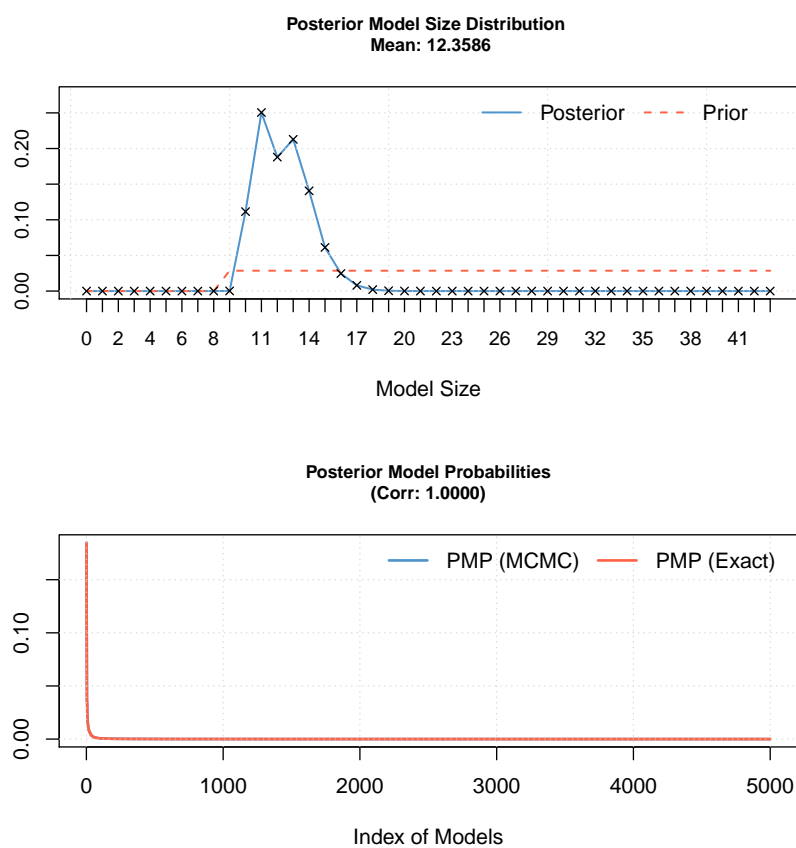
Figure B1: Model size and convergence
