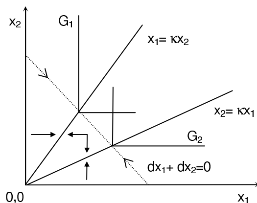
Figure 1: Mapping from inputs (x_1, x_2) to outputs (G_1, G_2)
