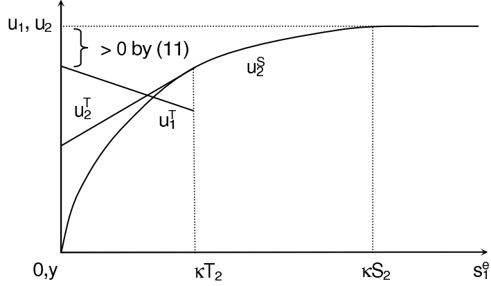
Figure 2: The utilities of the delegates for the best S-response and the best T-response of Delegate 2 to expected S-strategy of Delegate 1
