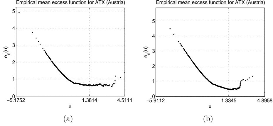
Figure 3: Empirical mean excess plot for the left tail (a) and the right tail (b) for the ATX (Austria) index.
