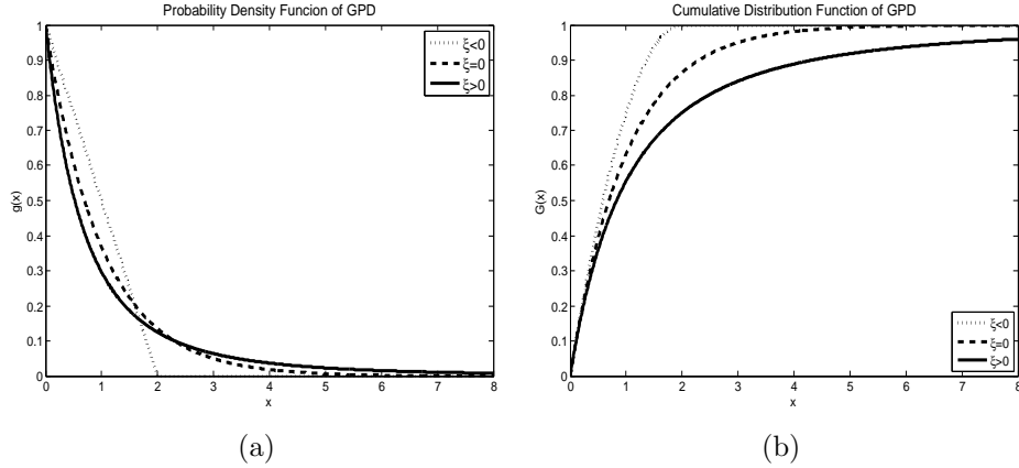
Figure 1: Probability density functions and cumulative distribution functions. \xi = 0 exponential, \xi = -0.5 Pareto type II and \xi = 0.5 Pareto distribution. In all cases \beta = 1 and \nu = 0 .
