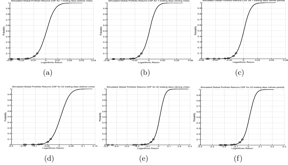
Figure 5: Empirical cumulative distribution function of simulated portfolio returns. Circles (from left to right) represent VaR estimates at 99.99%, 99.99%, 99.95%, 99.9%, 99.5%, 99%, 95% and 90% confidence intervals. [a-c] VaR estimation for 1 Day, [d-f] VaR estimation for 22 Days. [a,d] 2000-2004 (low volatility sample), [b,e] 2005-2009 (high volatility sample) and [c,f] 2000-2009 (whole sample).
