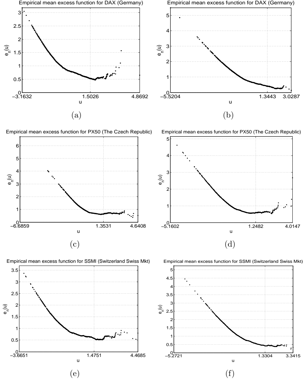
Figure B.6: Mean excess plot for the lower (left) tail [a-c-e] and upper (right) tail [b-d-f].
