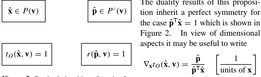
Figure 2: Dual relationships of a pair of polar points (\hat{\mathbf{p}}, \hat{\mathbf{x}})
