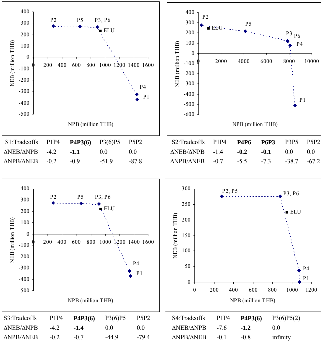
Figure 2. Approximated Pareto frontiers and tradeoff rates in various scenarios
