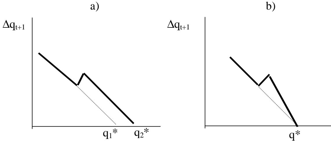
Figure 2.3 Hypothetical Market Change curves a) shifting q^* and b) shifting the value of \beta .
