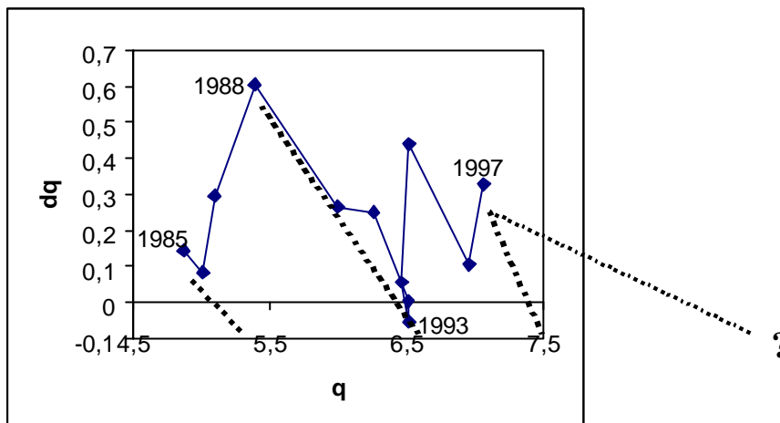
Figure 3.1. Market Change curve for Denmark
