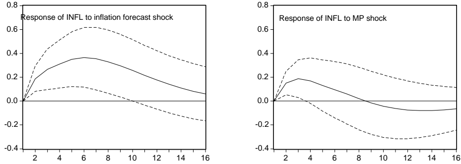
Figure 8: Response of inflation to news of future inflation and to a MP shock in a VAR including the forecast of future inflation from the ASA/NBER survey.
