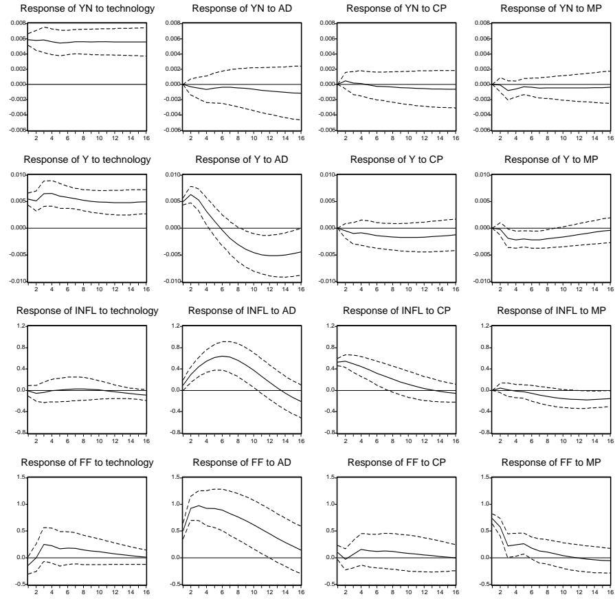
Figure 6: Impulse responses for the VAR: natural output, output, inflation, federal funds rate. Error bands include four standard deviations.
