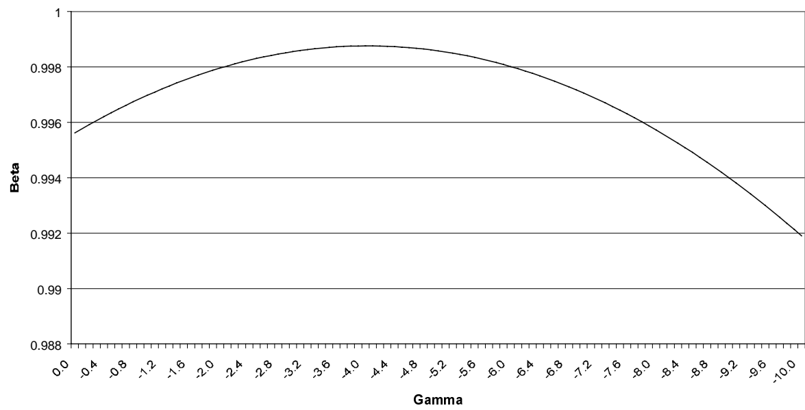
Figure 1. Combinations of beta and gamma for given parameter values: \alpha=0.001175 , \sigma=0.019678 , \rho=330.08
