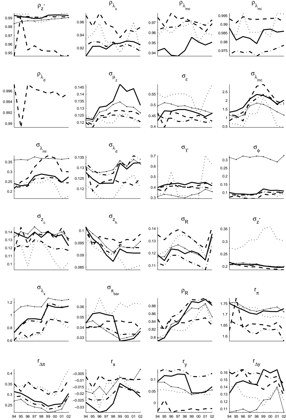
FIGURE 3. Sequential posterior mode estimates of the DSGE models' parameters using a year-by-year extended data set. DSGE diff. (—), DSGE count. ( \cdots ), Corr. mkup. (---), Var. cap. util. (- · -) and IID Markup (-+-).
