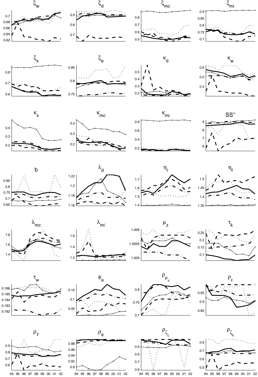
FIGURE 2. Sequential posterior mode estimates of the DSGE models' parameters using a year-by-year extended data set. DSGE diff. (—), DSGE point. ( \cdots ), Corr. mkup. (---), Var. cap. util. (- · -) and IID Markup (-+-).
