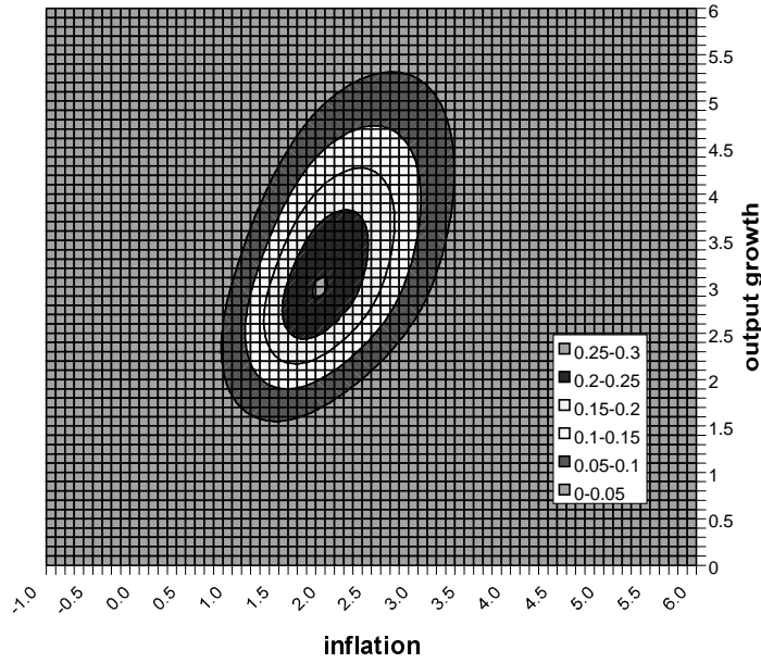
Figure 2b. Bivariate distribution surface
