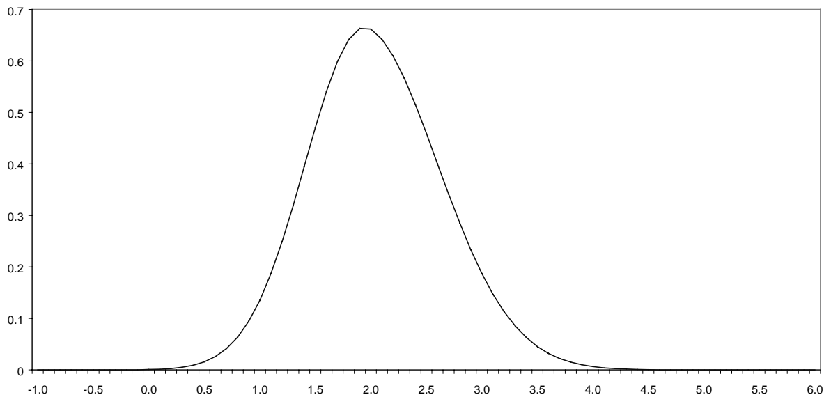
Figure 3a. Inflation distribution conditional on 3% output growth
