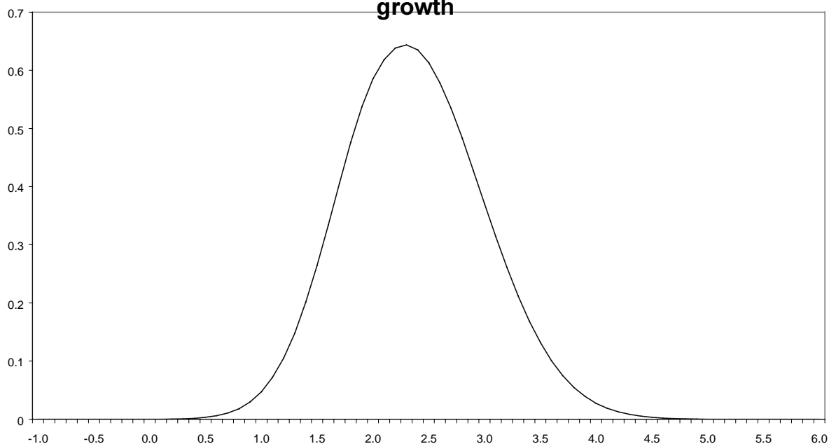
Figure 3b. Inflation distribution conditional on 4% output growth
