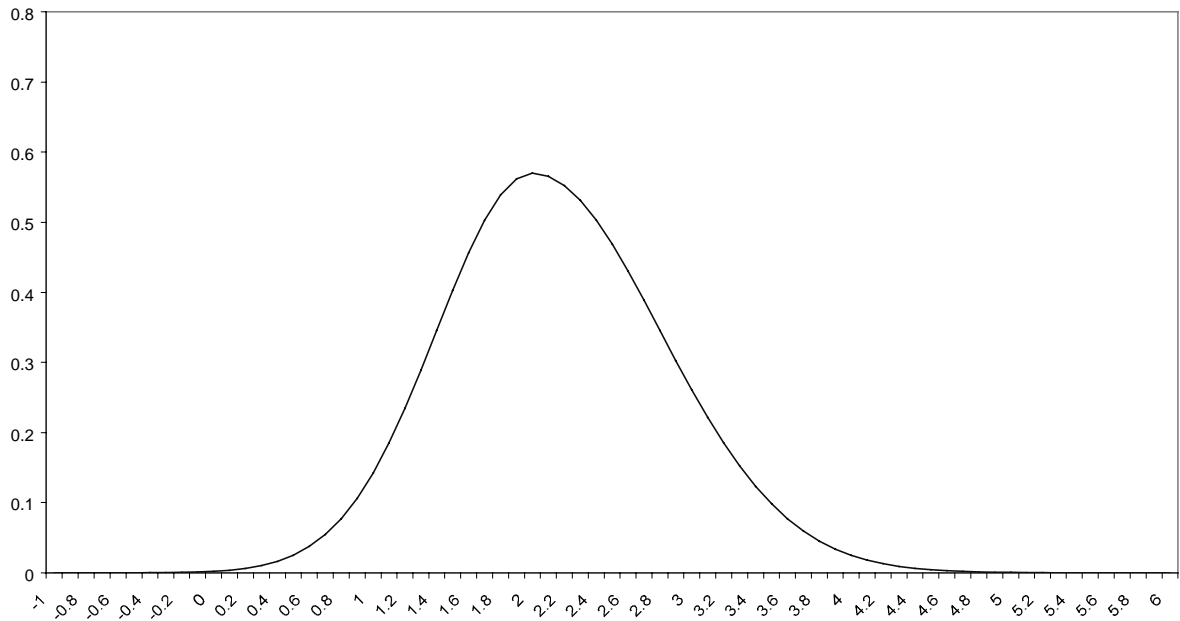
Figure 1. Marginal distribution for inflation forecast
