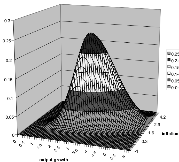
Figure 2a. Bivariate distribution for output and inflation
