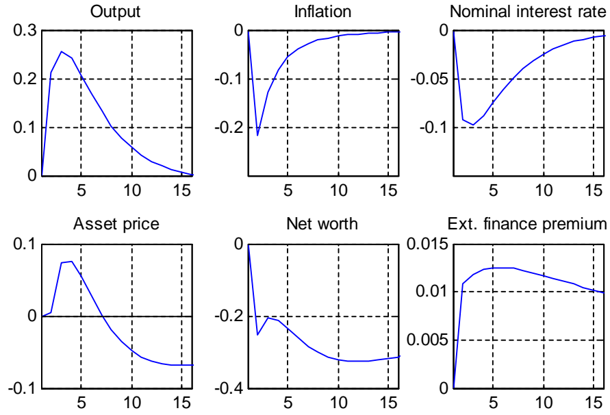
Figure 3: Positive technology shock, symmetric policy reaction to asset prices ( \phi_q = 0.5 )
