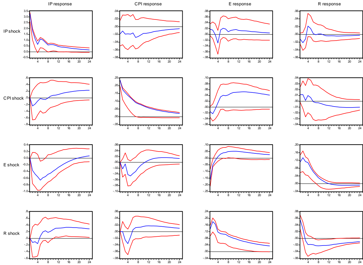
Figure 4: Impulse response functions with bootstrapped 90% confidence bounds
