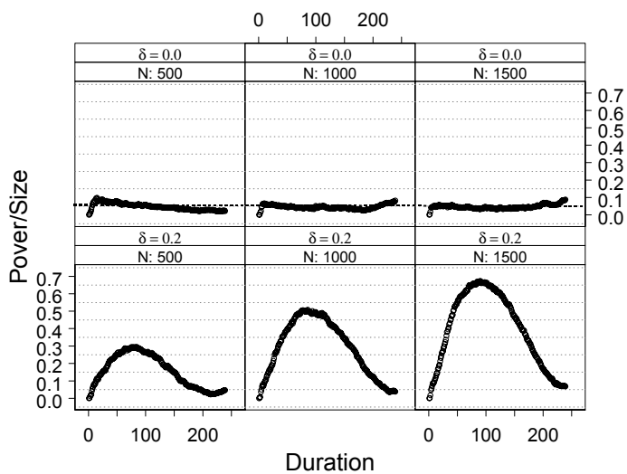
Figure 3: The power of the Wald test based on the \hat{\Delta}(t) estimator with and evaluation period of \bar{L} = 240 months.
