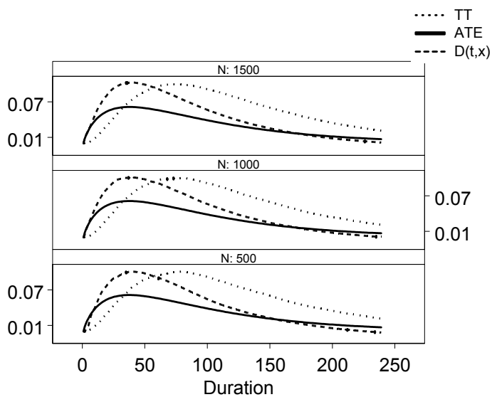
Figure 2: \hat{\Delta}_1(t) = D(t, x) , ATE and TT with a treatment ( \delta = 0.2 ) and evaluation period of \bar{L} = 240 months.
