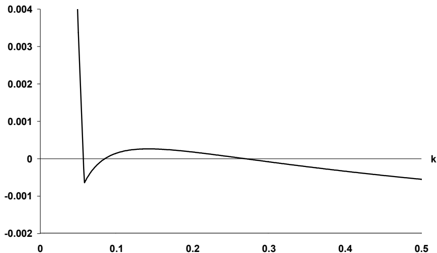
Figure 1: Numerical example of multiple equilibria
