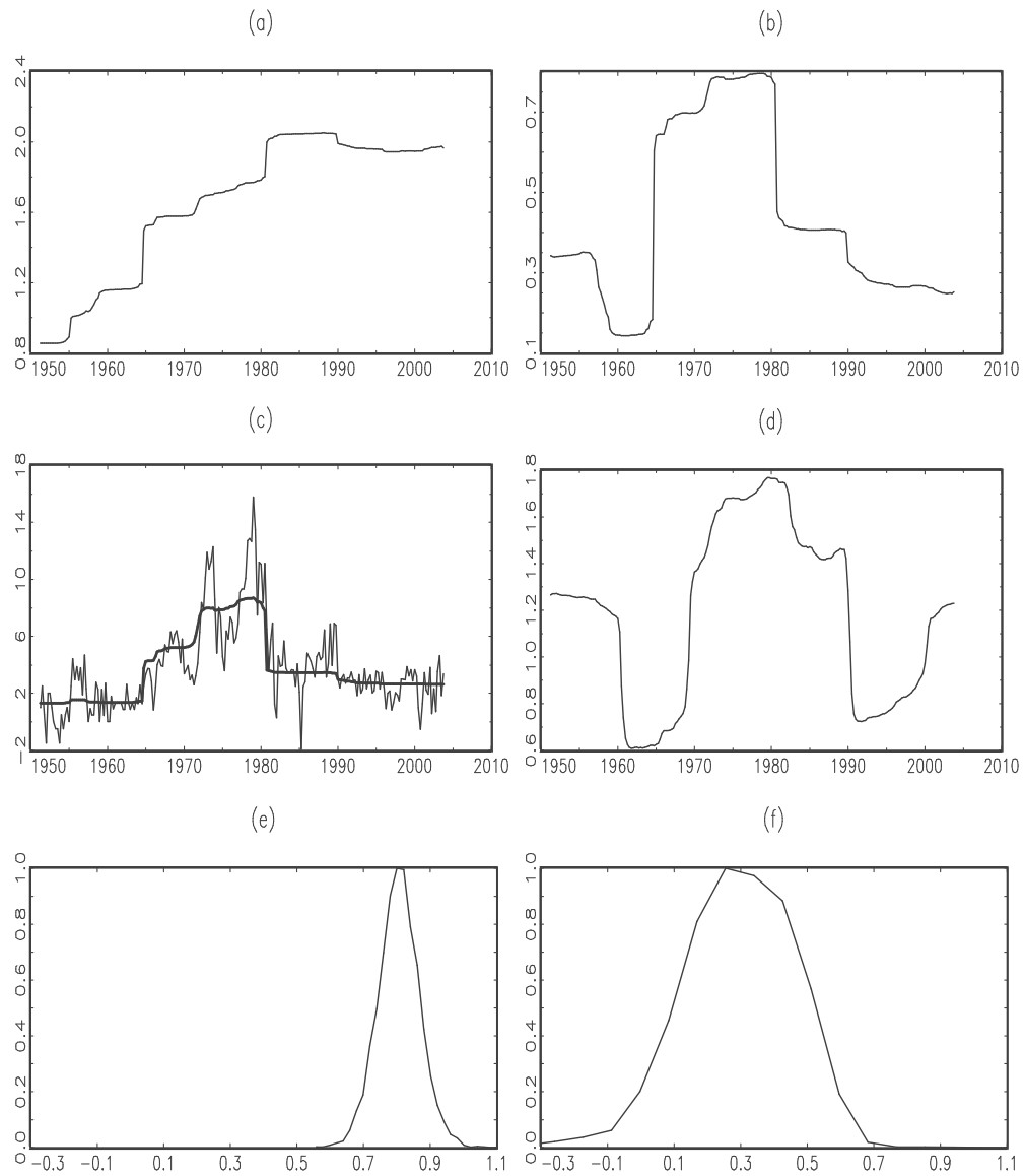
Figure 2: AR(1) model of U.S. inflation: (a) posterior mean of c_t (b) posterior mean of b_t (c) inflation and posterior median of c_t/(1-b_t) (d) posterior mean of \sigma_t (e) posterior distribution of b_{1979Q1} (f) posterior distribution of b_{2004Q4} .
