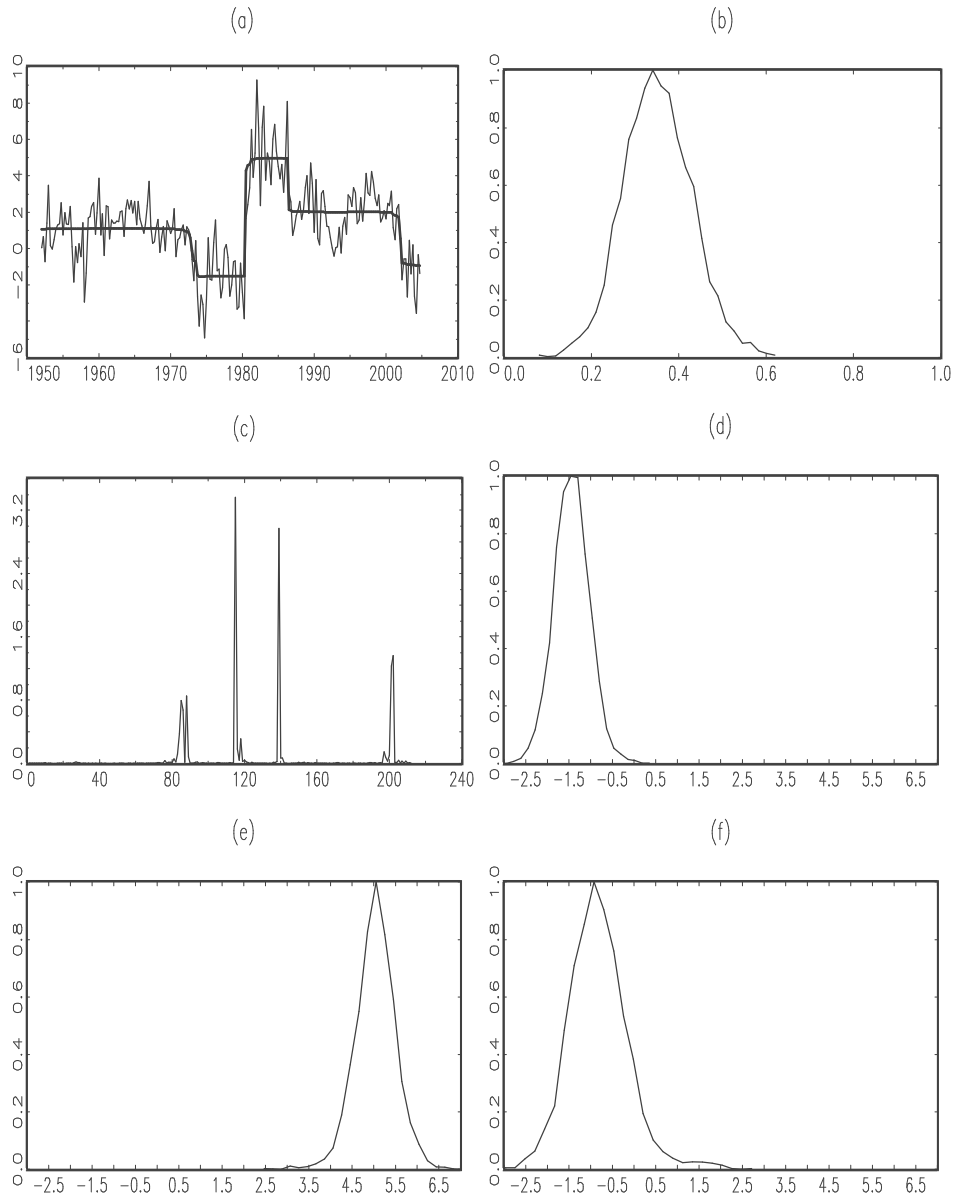
Figure 1: AR(1) model with mean shifts for the U.S. real interest rate. (a) real interest rate and posterior mean of \mu_t (b) posterior density of \rho (c) posterior mean of K_{m,t} (d) posterior distribution of \mu_{1976Q1} (e) posterior distribution of \mu_{1982Q1} (f) posterior distribution of \mu_{2004Q4} .
