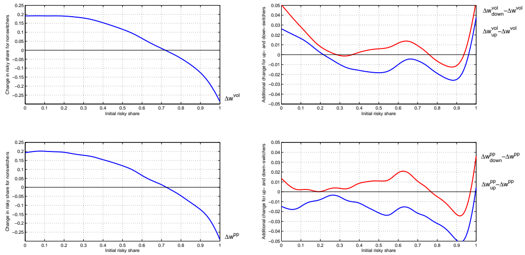
Figure 3: Fitted active changes for up-, down-, and non-switchers
