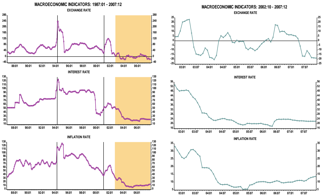
Figure.3: Behaviour of the Trend-Cycle Components
