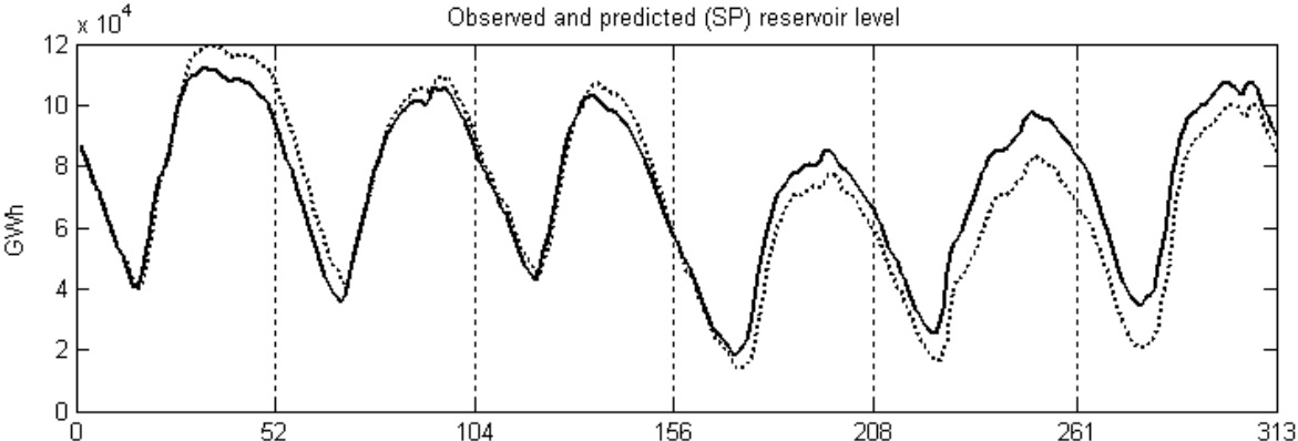
Figure 4: Observed (solid) vs. simulated (dashed) reservoirs (Kauppi and Liski 2008)
