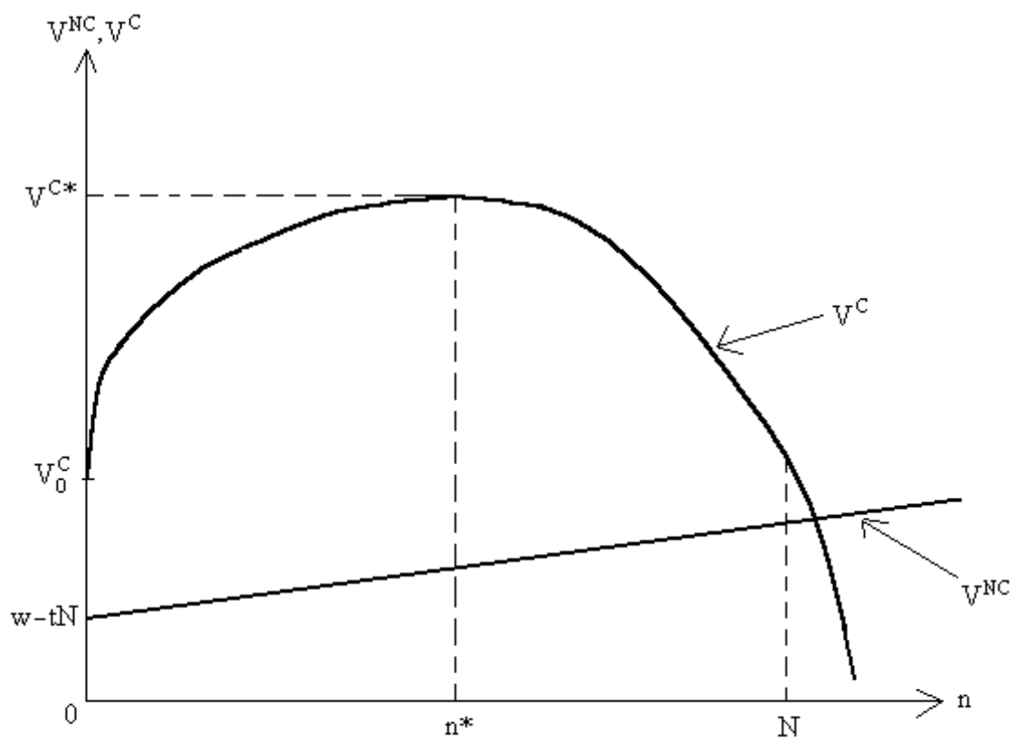
Figure 2: Total-Crime Equilibrium
