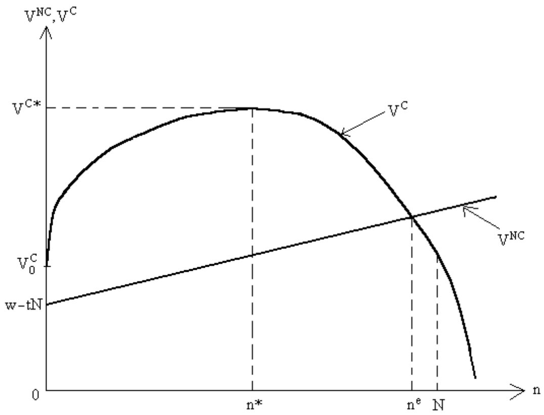
Figure 3: Crime-Ridden Equilibrium
