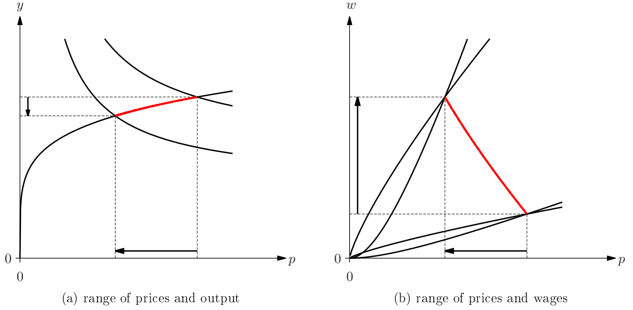
Figure 11: Output, prices, and wages for \lambda from zero to one
