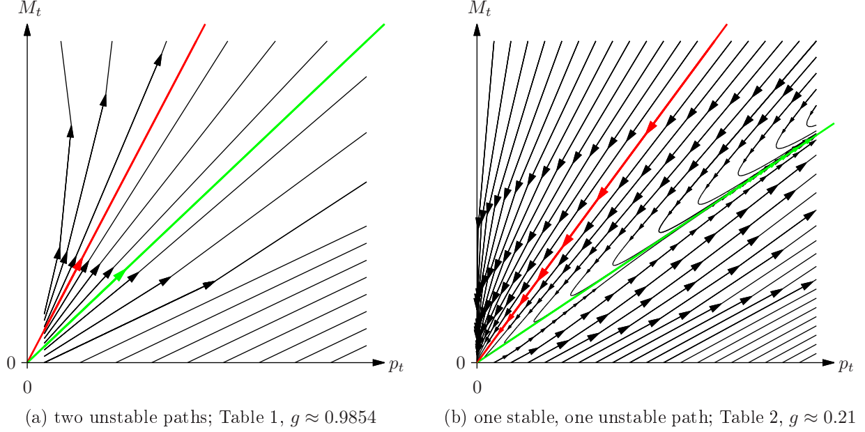
Figure 20: Stability of balanced paths in state space
