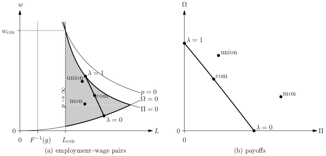
Figure 14: Wages, employment, and payoffs under low price expectations
