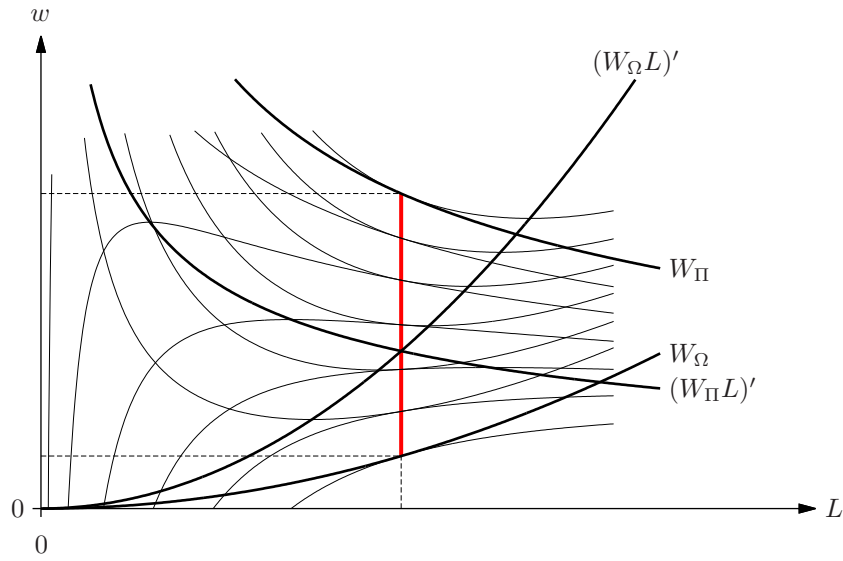
Figure 1: Determining the level of employment
