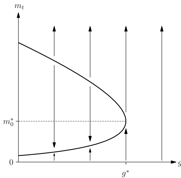
Figure 19: Balanced paths and the role of government consumption
