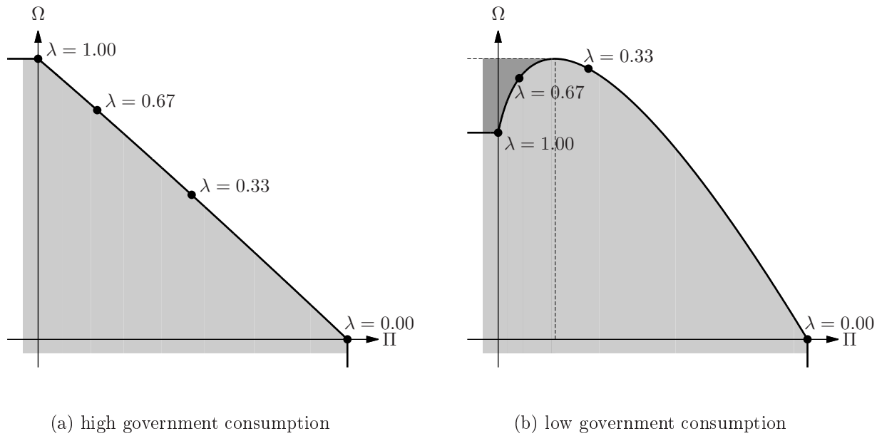
Figure 7: Net wage bill and profit with price feedback
