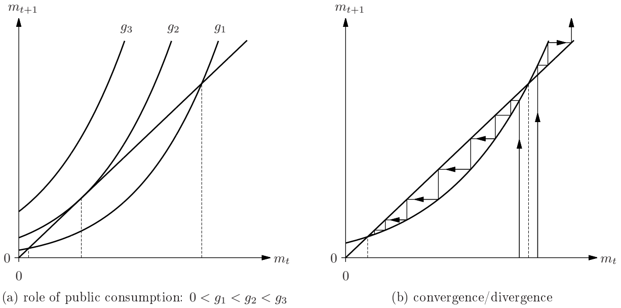
Figure 17: Existence, uniqueness, and stability
