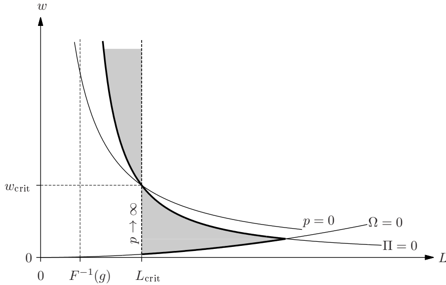
Figure 13: Employment–wage pairs under individual rationality and feasibility
