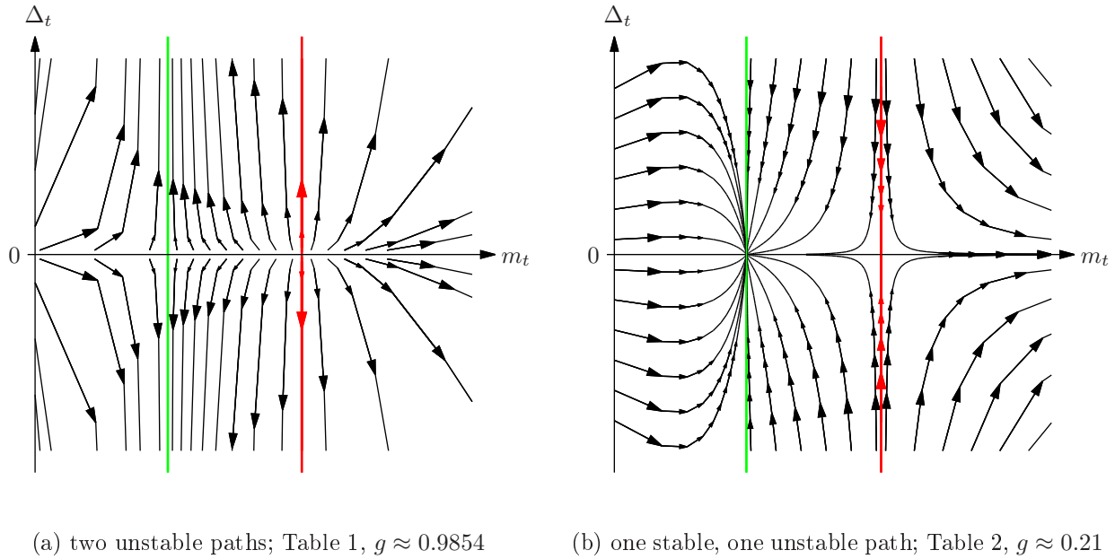
Figure 21: Stability of balanced paths in (\Delta, m) -space
