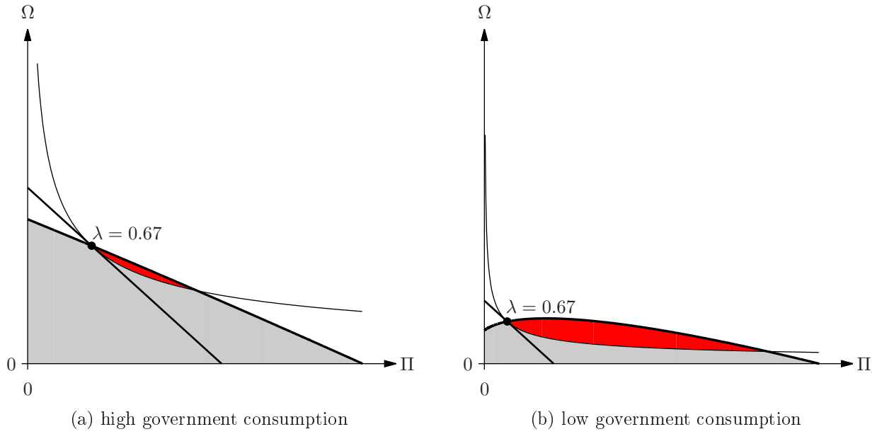
Figure 9: No efficient Nash bargaining solution under price feedback: the better set (red)
