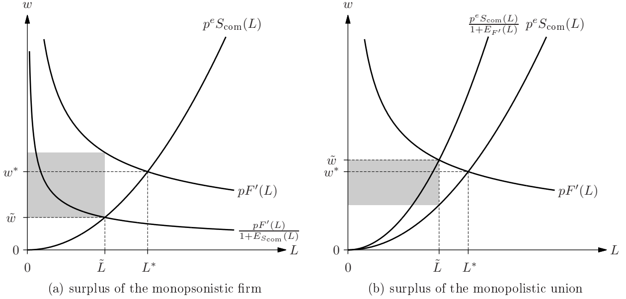
Figure 3: Wages, employment, and surplus in monopsonistic situations; (p^e, p) given
