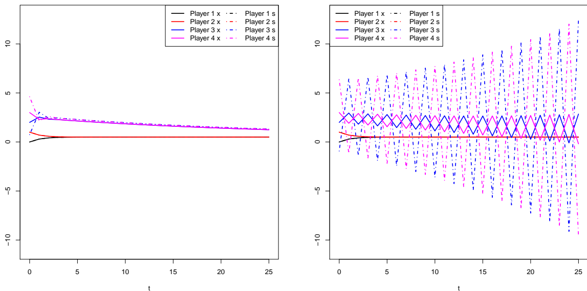
Figure 4: The opinion dynamics of Example 2 for (a) \delta_{ROTW} = -.7 and (b) \delta_{ROTW} = -.92 .
